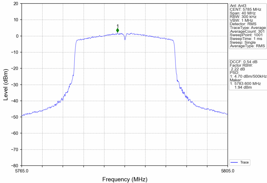
802.11ax(HEW20)_MCH_5785MHz_RU242_Left_MIMO_NTNV
