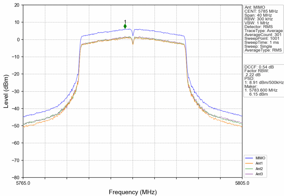
802.11ax(HEW20)_MCH_5785MHz_RU242_Left_MIMO_NTNV
