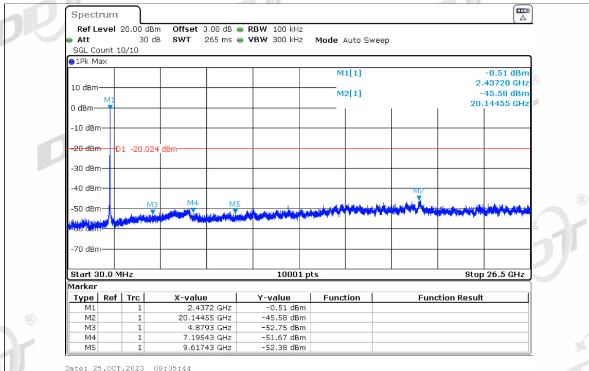
Tx. Spurious NVNT g 2437MHz Ant2 Ref
