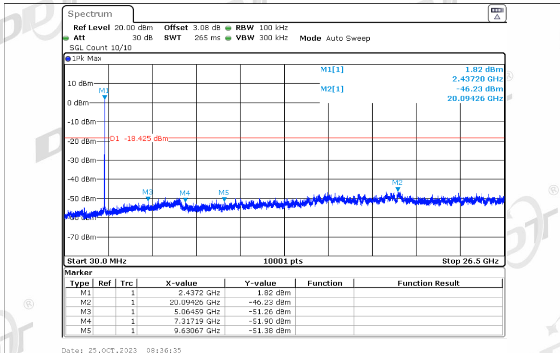
Tx. Spurious NVNT b 2437MHz Ant2 Ref
