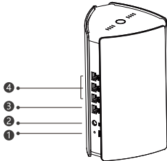
1 Reset button 2 Power port 3 WAN port 4 LAN1-2 port
