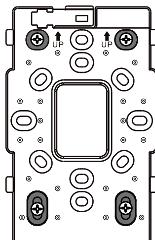
Bracket on South African-standard 114 mm × 114 mm Junction Box
