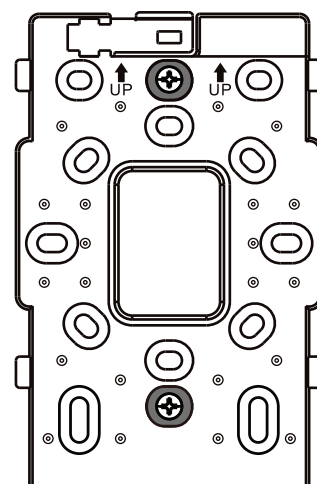
Bracket on American-standard 108 mm × 59 mm Junction Box
