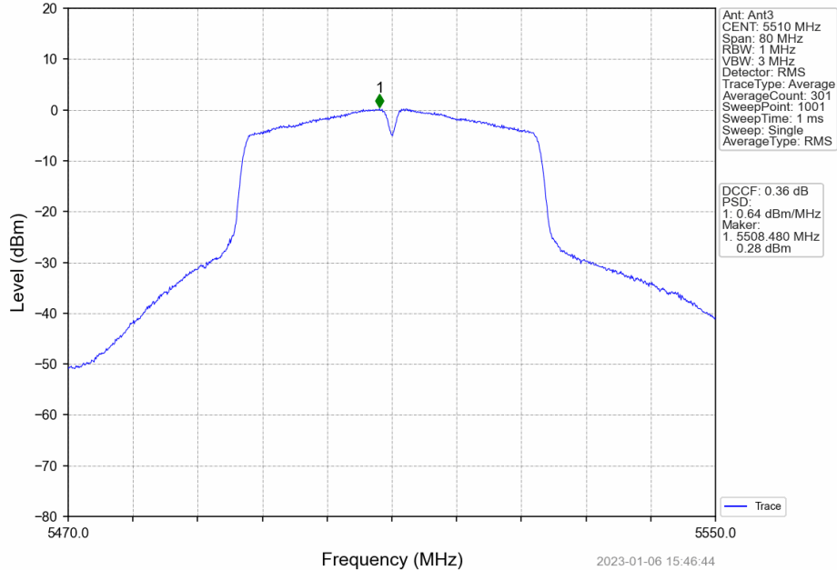
802.11ac(VHT40)_LCH_5510MHz_MIMO_NTNV
