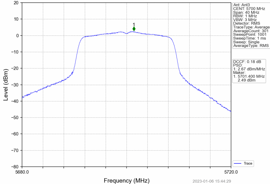
802.11ac(VHT20)_HCH_5700MHz_MIMO_NTNV
