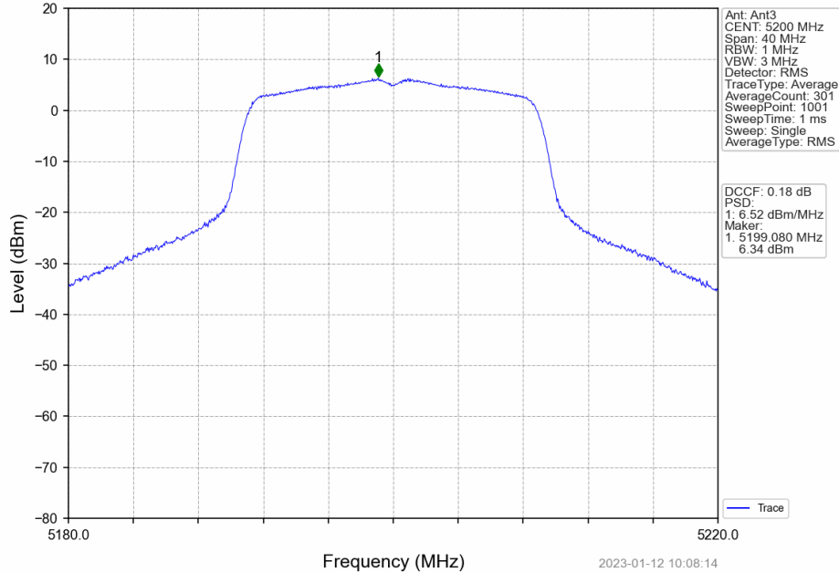
802.11ac(VHT20)_MCH_5200MHz_MIMO_NTNV
