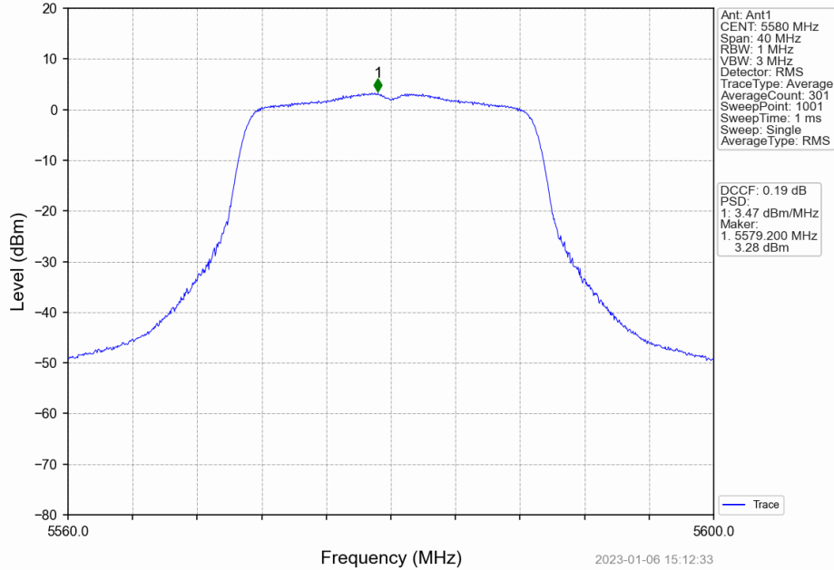
802.11n(HT20)_MCH_5580MHz_Ant2_NTNV
