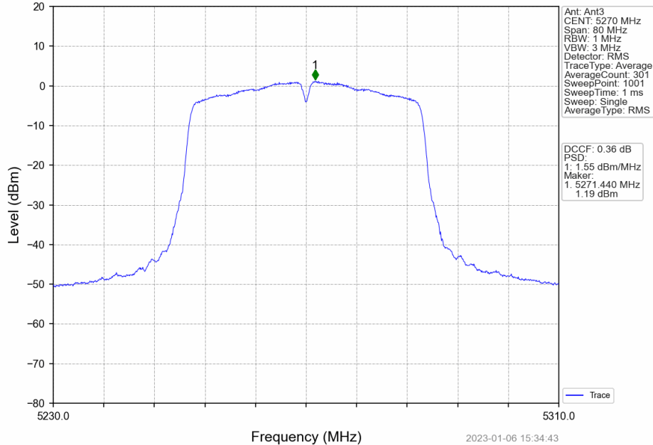
802.11ac(VHT40)_LCH_5270MHz_MIMO_NTNV
