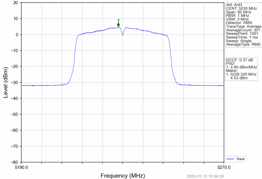
802.11n(HT40)_HCH_5230MHz_MIMO_NTNV
