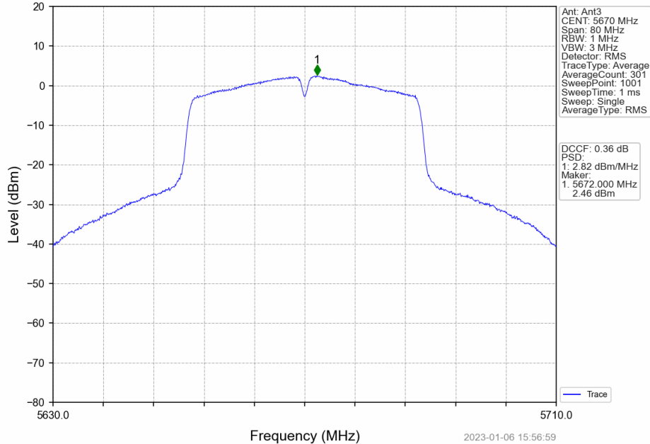
802.11ac(VHT40)_HCH_5670MHz_MIMO_NTNV
