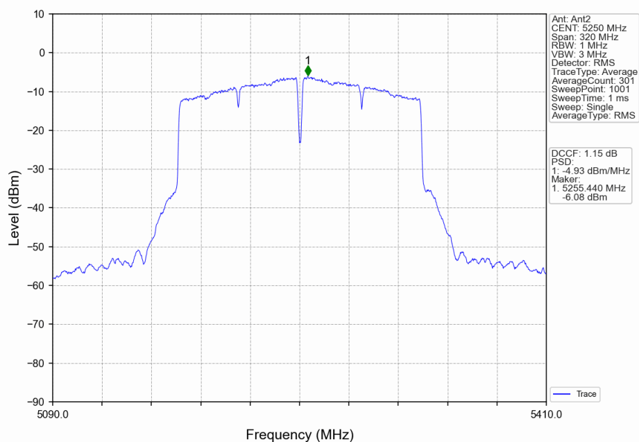
802.11ac(VHT160)_MCH_5250MHz_Ant2_NTNV
