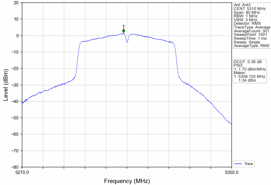
802.11ac(VHT40)_HCH_5310MHz_MIMO_NTNV
