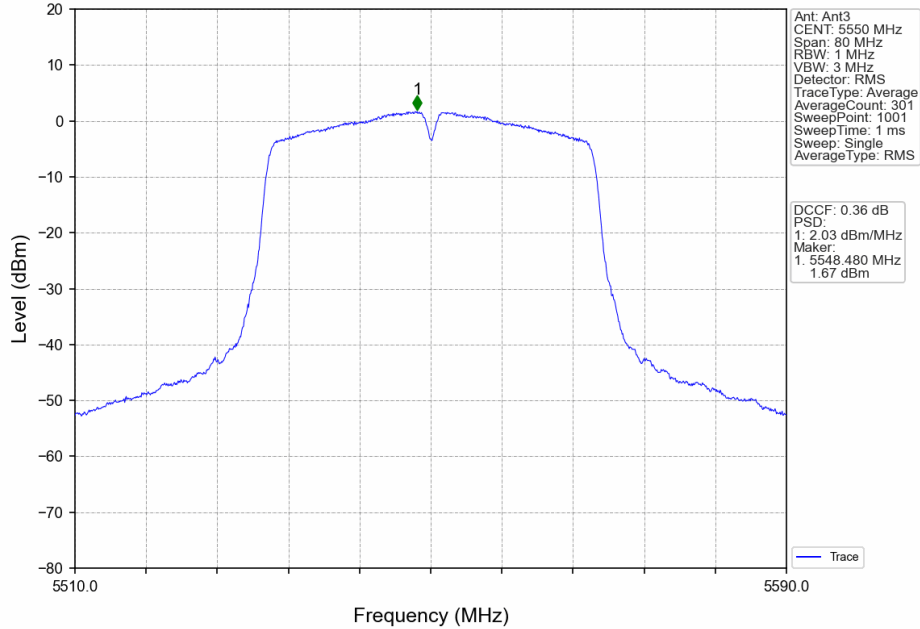
802.11ac(VHT40)_MCH_5550MHz_MIMO_NTNV
