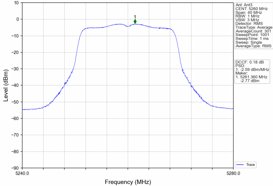
802.11ac(VHT20)_LCH_5260MHz_MIMO_NTNV
