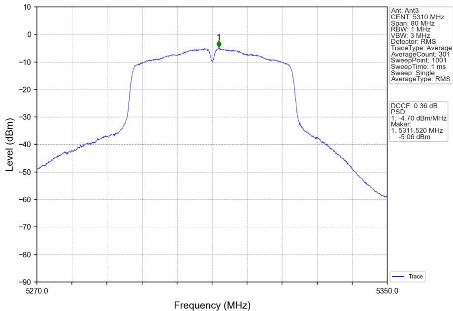
802.11n(HT40)_HCH_5310MHz_MIMO_NTNV
