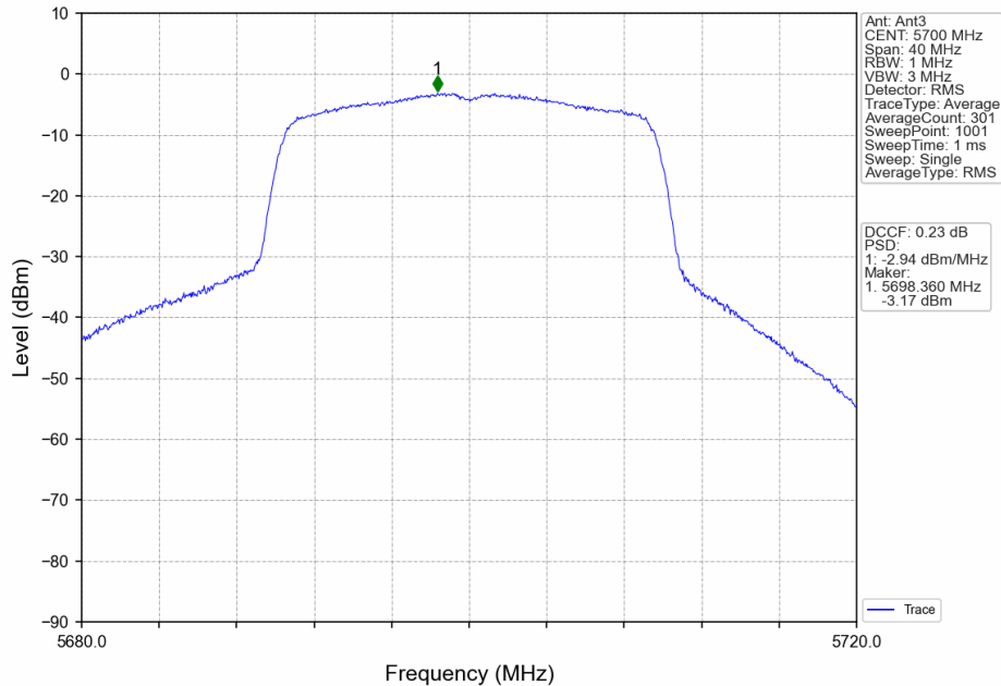
802.11ax(HEW20)_HCH_5700MHz_RU242_Left_MIMO_NTNV
