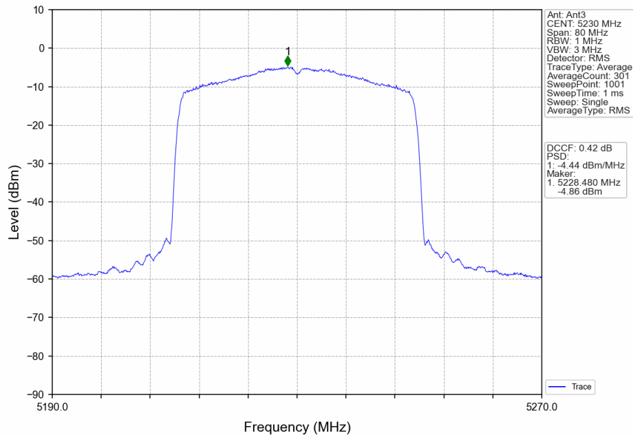
802.11ax(HEW40)_HCH_5230MHz_RU484_Left_MIMO_NTNV
