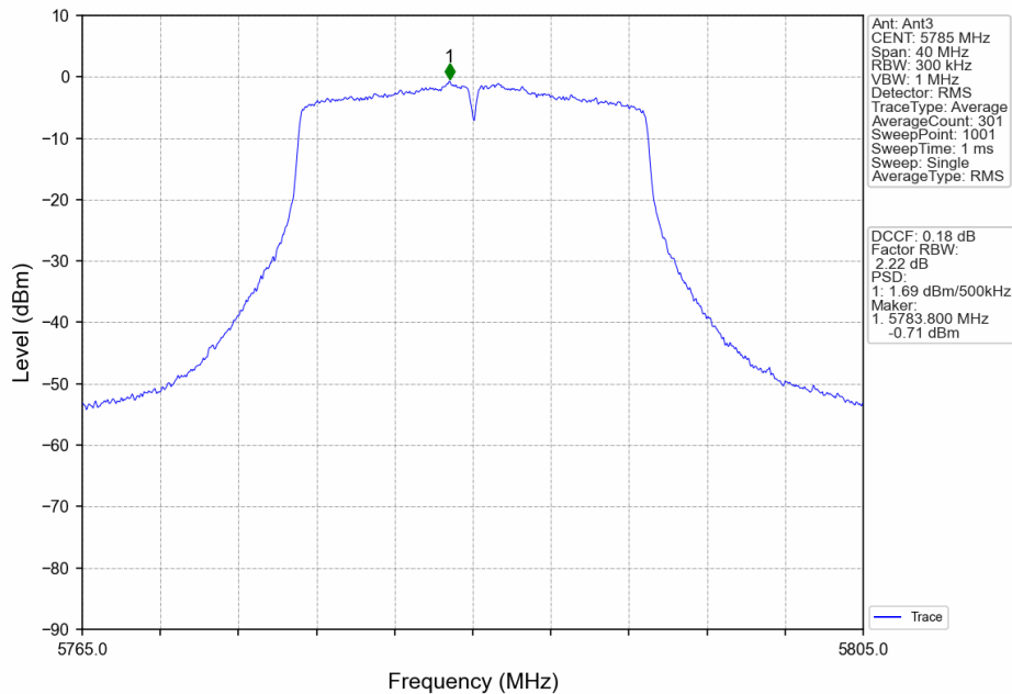
802.11ac(VHT20)_MCH_5785MHz_MIMO_NTNV
