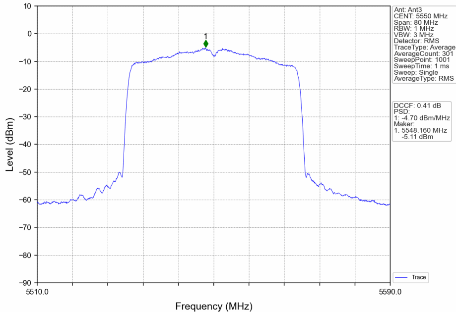
802.11ax(HEW40)_MCH_5550MHz_RU484_Left_MIMO_NTNV
