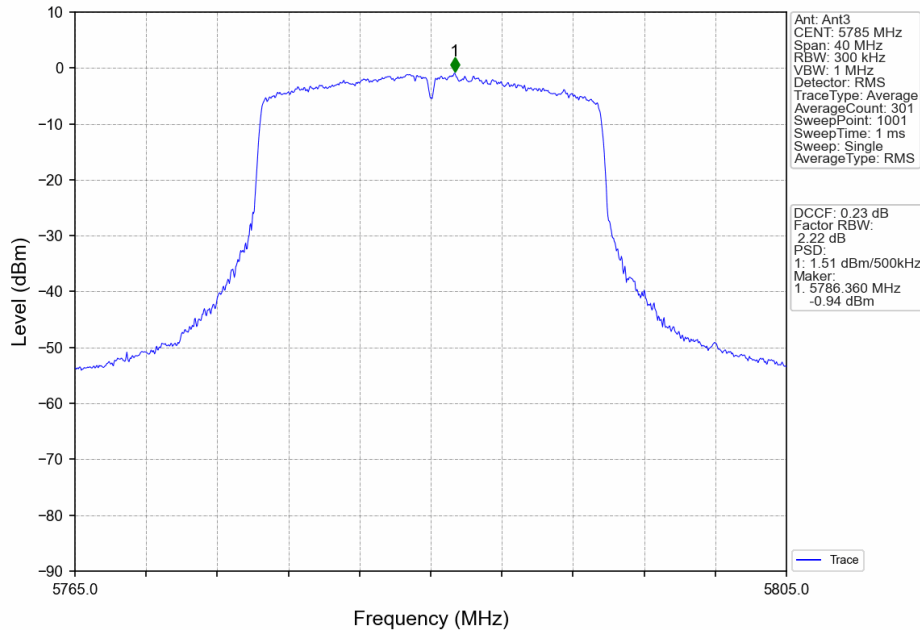
802.11ax(HEW20)_MCH_5785MHz_RU242_Left_MIMO_NTNV
