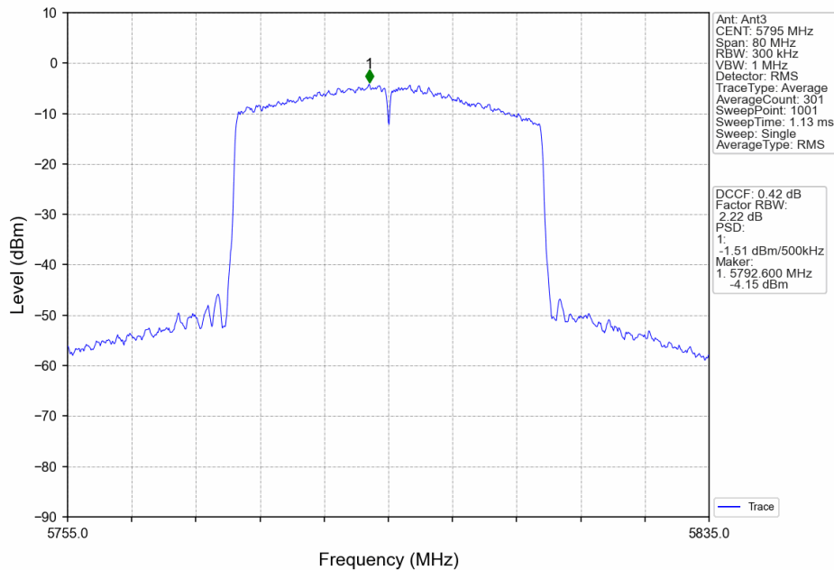
802.11ax(HEW40)_HCH_5795MHz_RU484_Left_MIMO_NTNV
