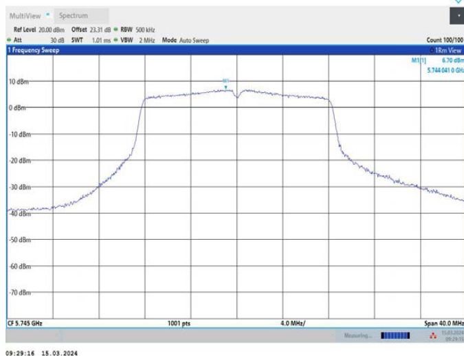
11A_Ant3_5745
