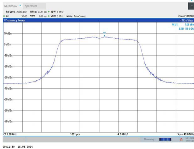
11A_Ant3_5580
