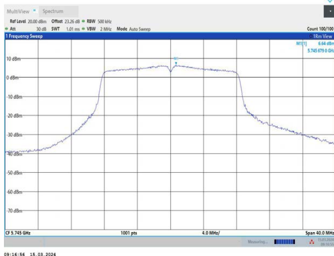
11A_Ant3_5745
