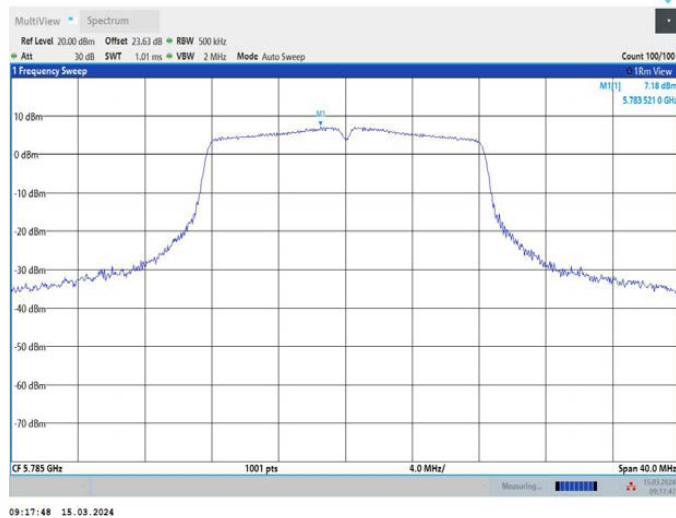
11A_Ant3_5785
