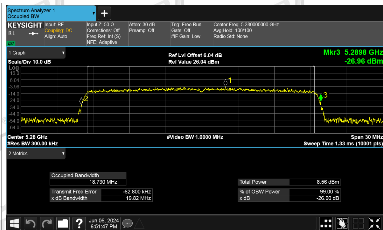
-26dB Bandwidth NVNT be20 5280MHz Ant3
