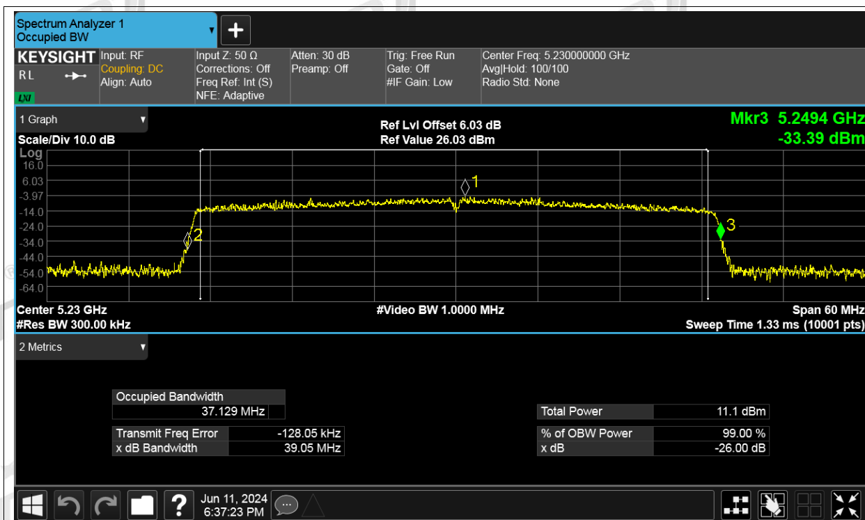
-26dB Bandwidth NVNT be40 5230MHz Ant3
