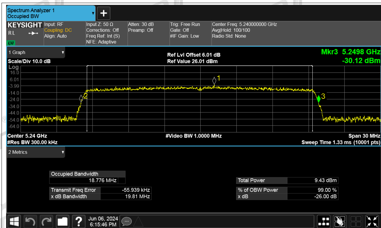
-26dB Bandwidth NVNT be20 5240MHz Ant3
