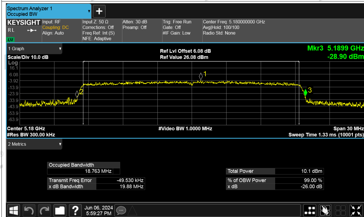
-26dB Bandwidth NVNT be20 5180MHz Ant2
