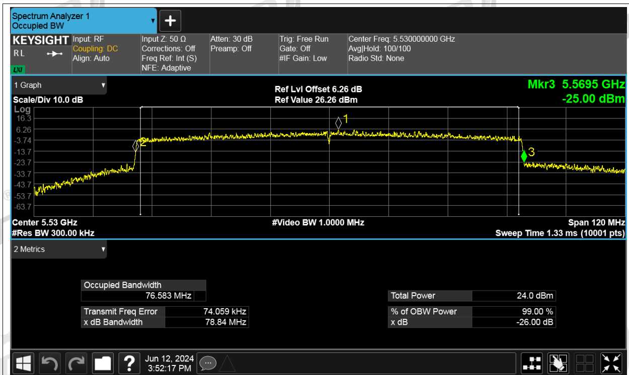
-26dB Bandwidth NVNT ax80 5530MHz Ant3
