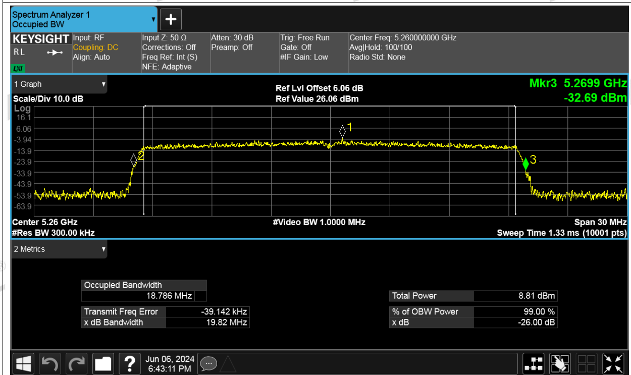
-26dB Bandwidth NVNT be20 5260MHz Ant3
