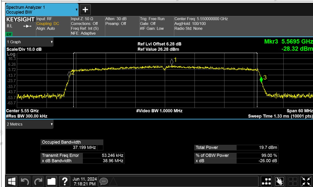
-26dB Bandwidth NVNT be40 5550MHz Ant2
