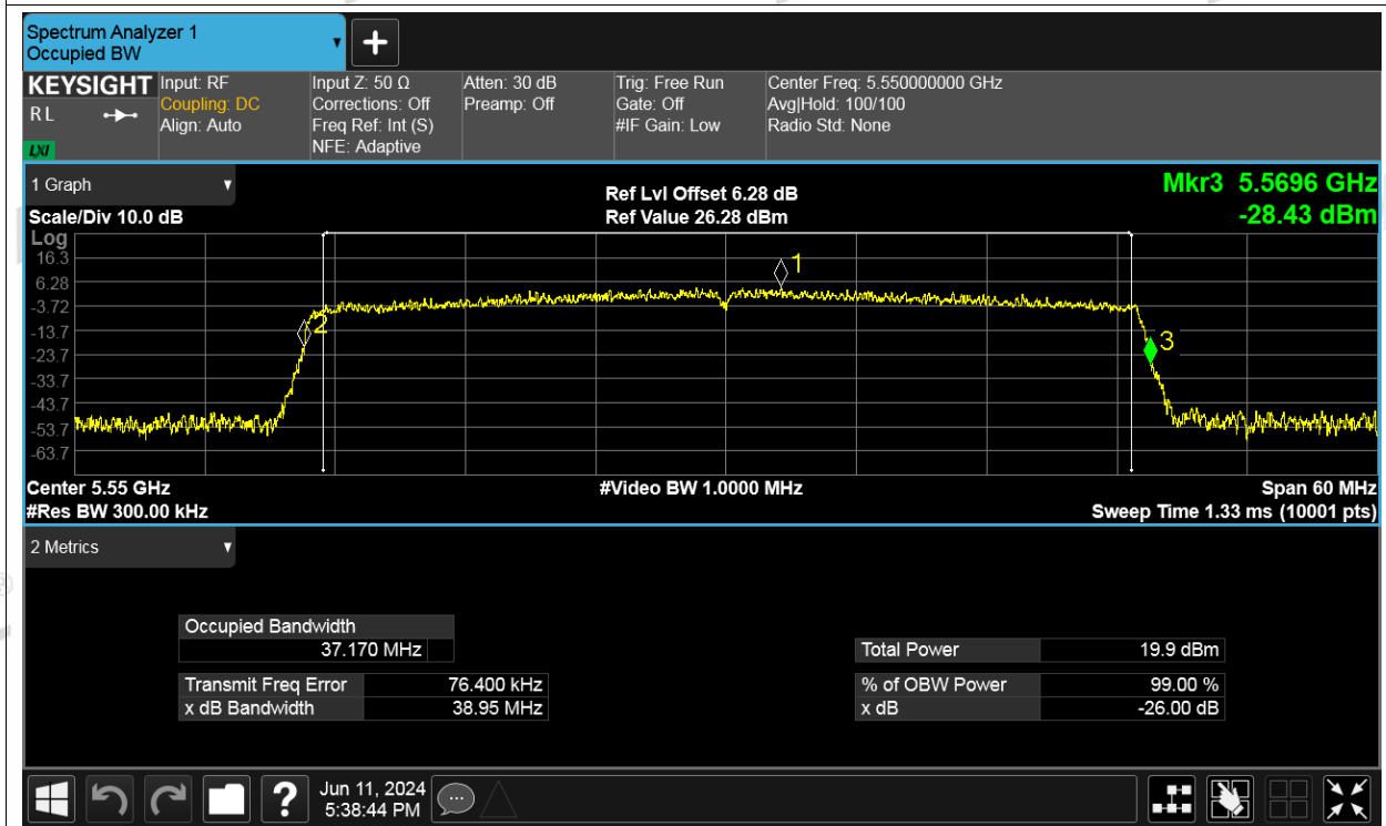
-26dB Bandwidth NVNT ax40 5550MHz Ant2
