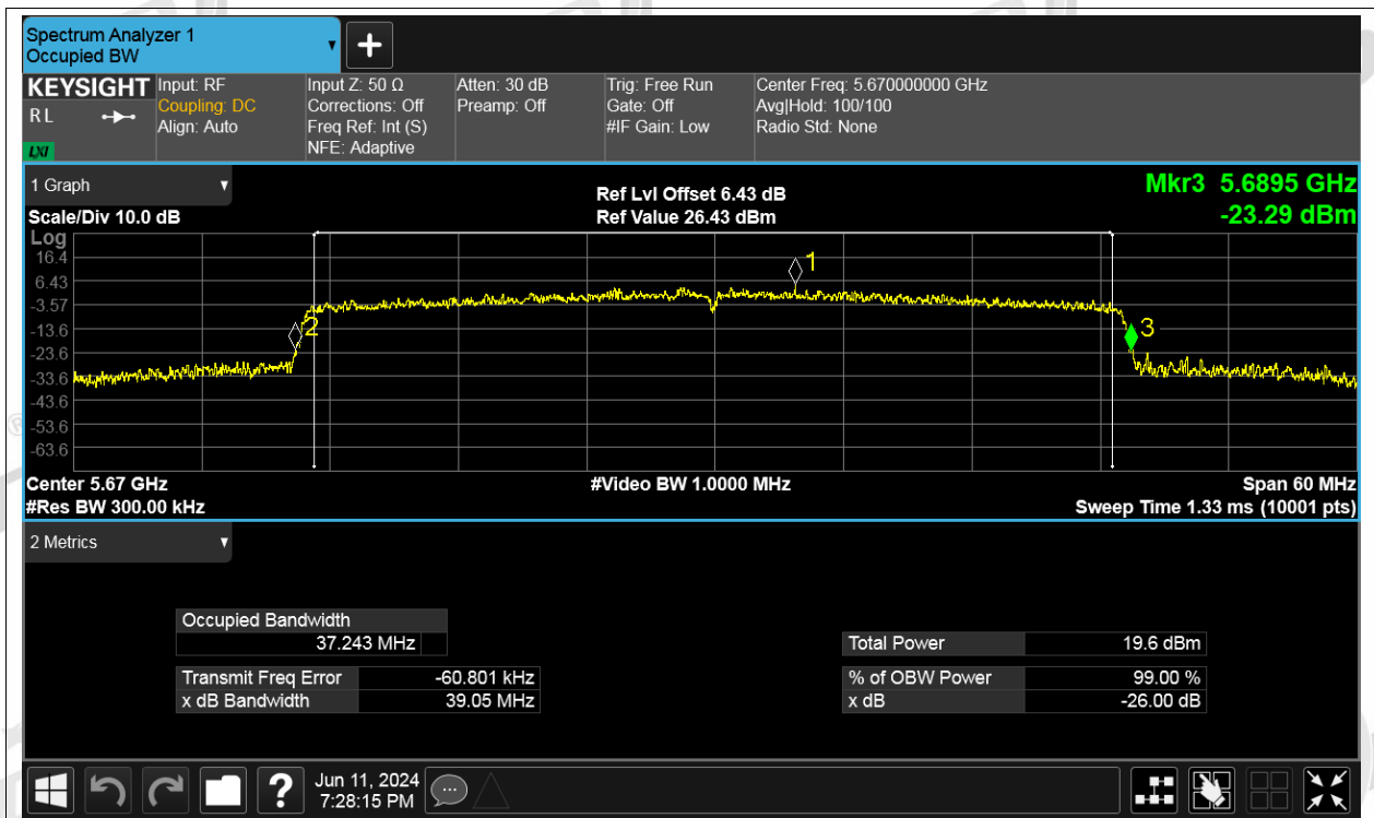
-26dB Bandwidth NVNT be40 5670MHz Ant2
