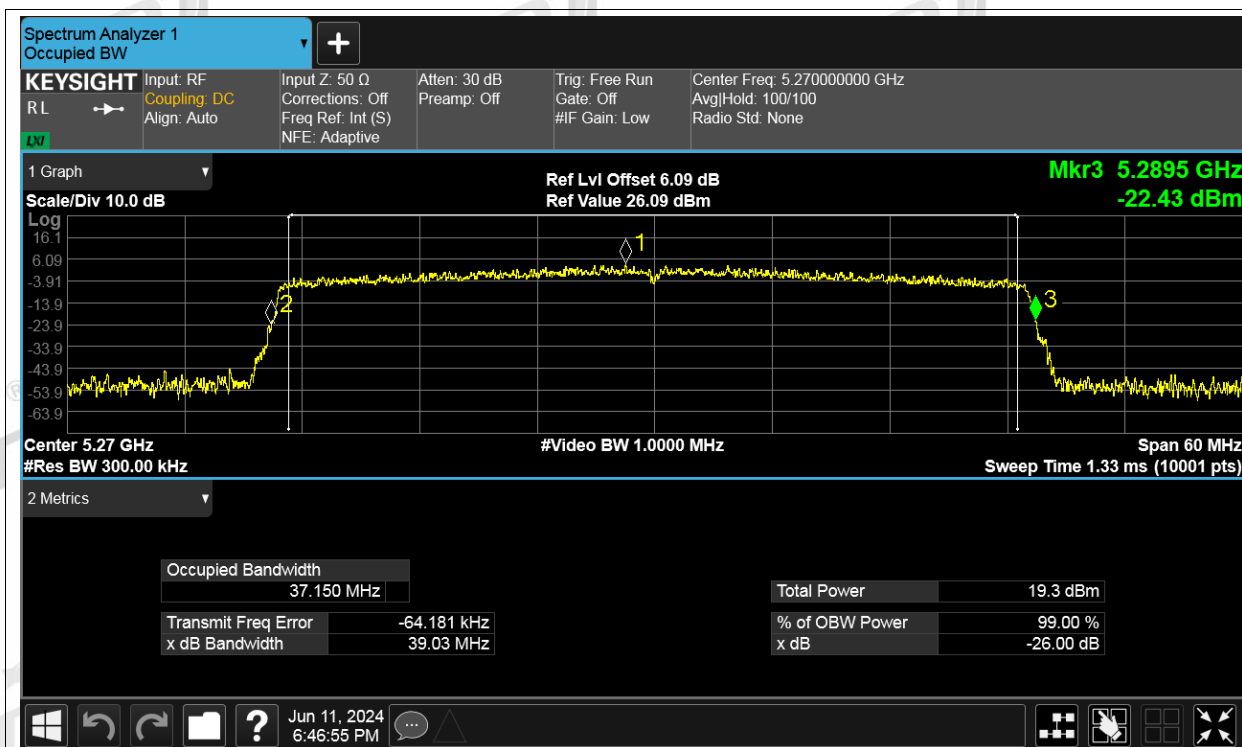
-26dB Bandwidth NVNT be40 5270MHz Ant2
