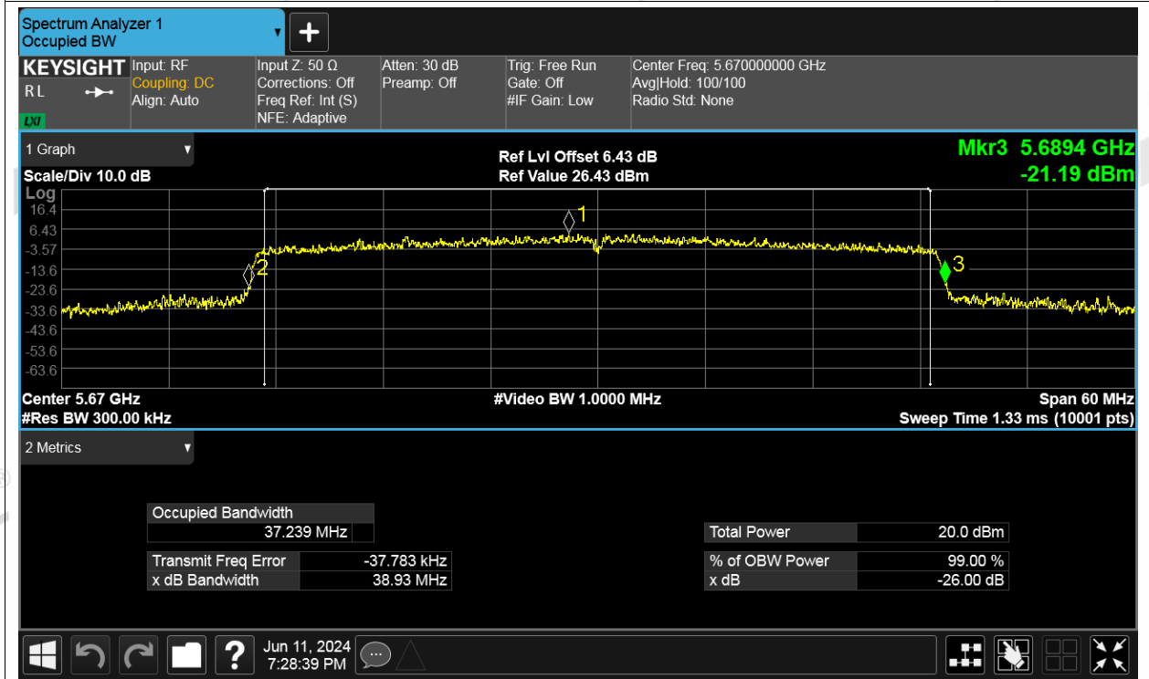
-26dB Bandwidth NVNT be40 5670MHz Ant3
