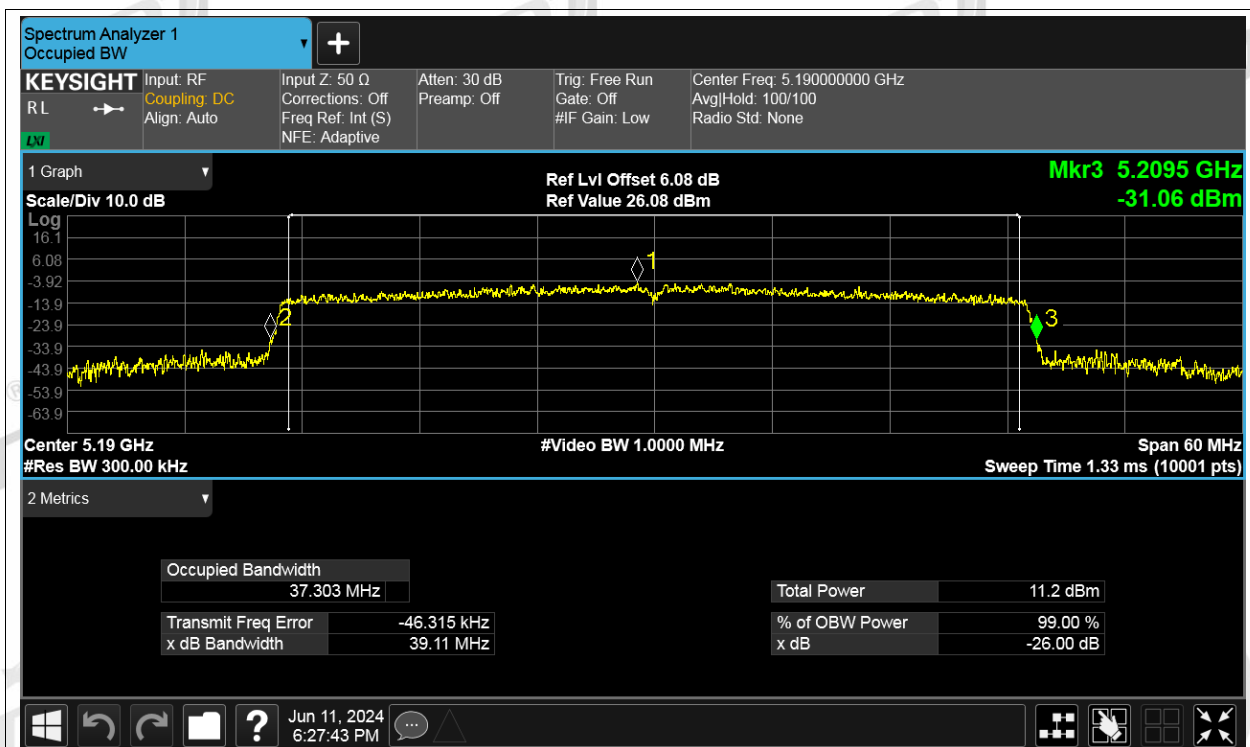
-26dB Bandwidth NVNT be40 5190MHz Ant2
