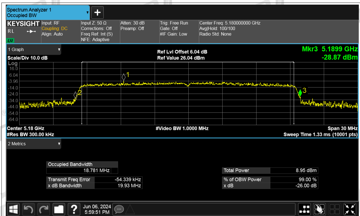
-26dB Bandwidth NVNT be20 5180MHz Ant3
