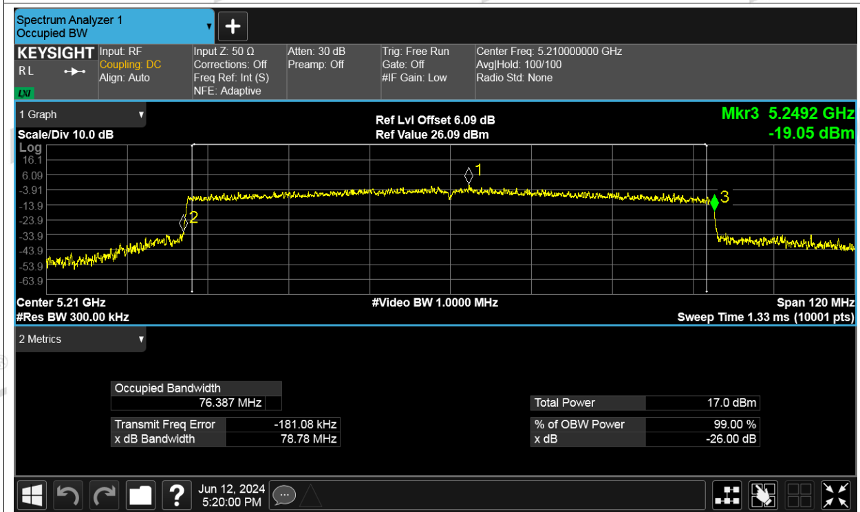
-26dB Bandwidth NVNT be80 5210MHz Ant2
