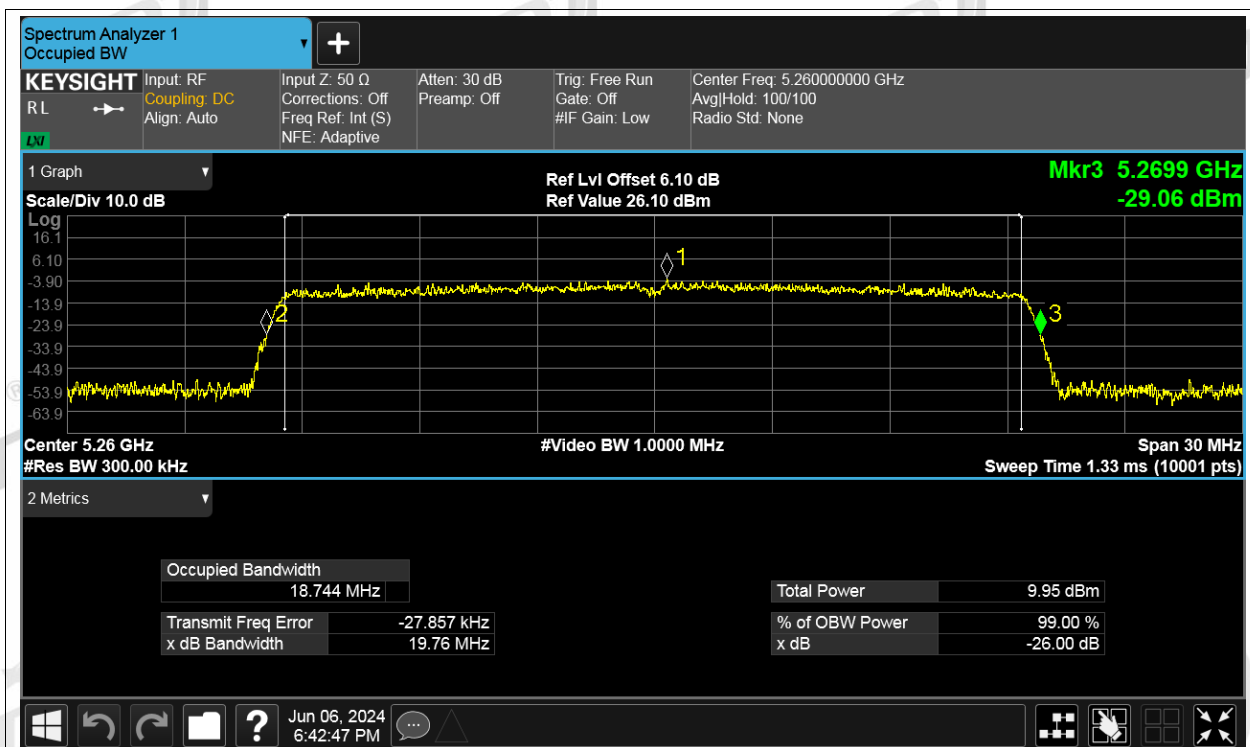
-26dB Bandwidth NVNT be20 5260MHz Ant2
