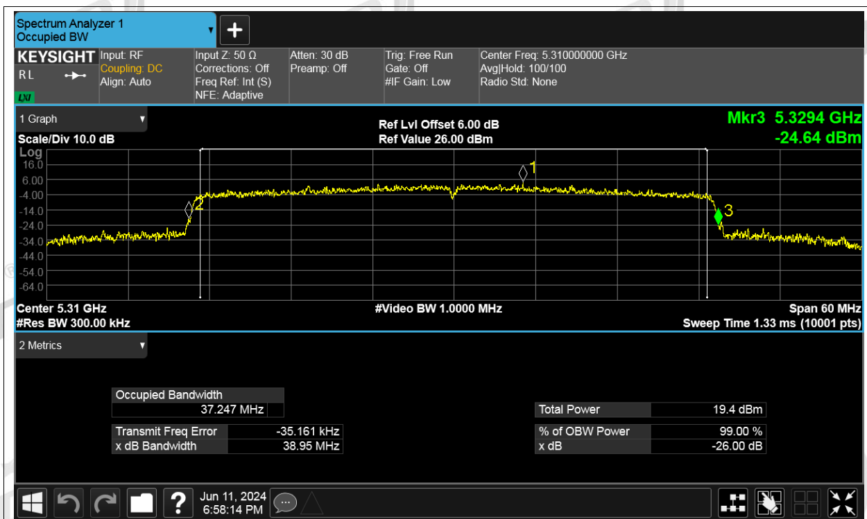
-26dB Bandwidth NVNT be40 5310MHz Ant3
