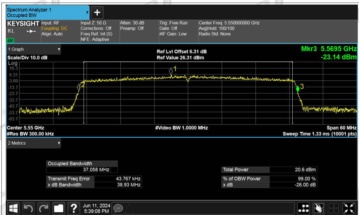
-26dB Bandwidth NVNT ax40 5550MHz Ant3
