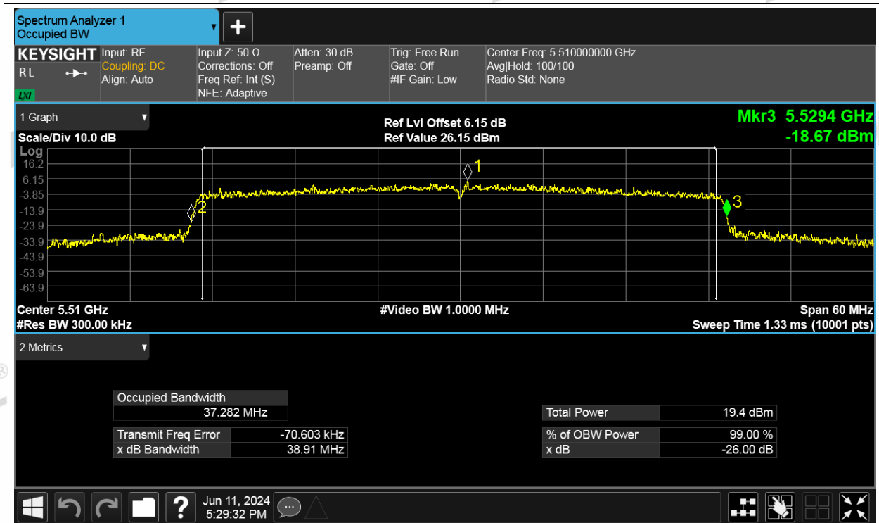
-26dB Bandwidth NVNT ax40 5510MHz Ant3
