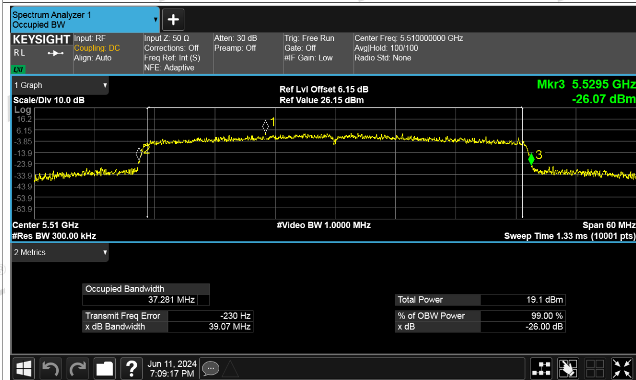
-26dB Bandwidth NVNT be40 5510MHz Ant3
