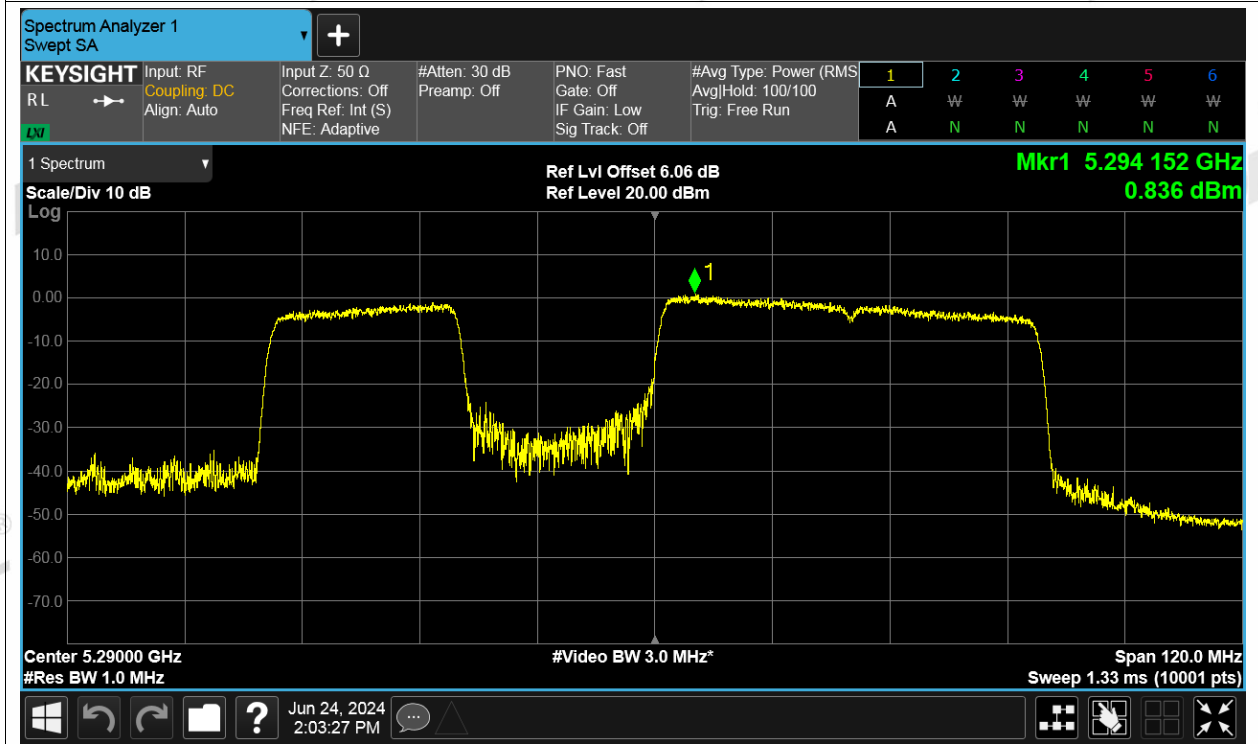
PSD NVNT be80 484+242-tone in a non-OFDMA MRU2 5290MHz Ant3
