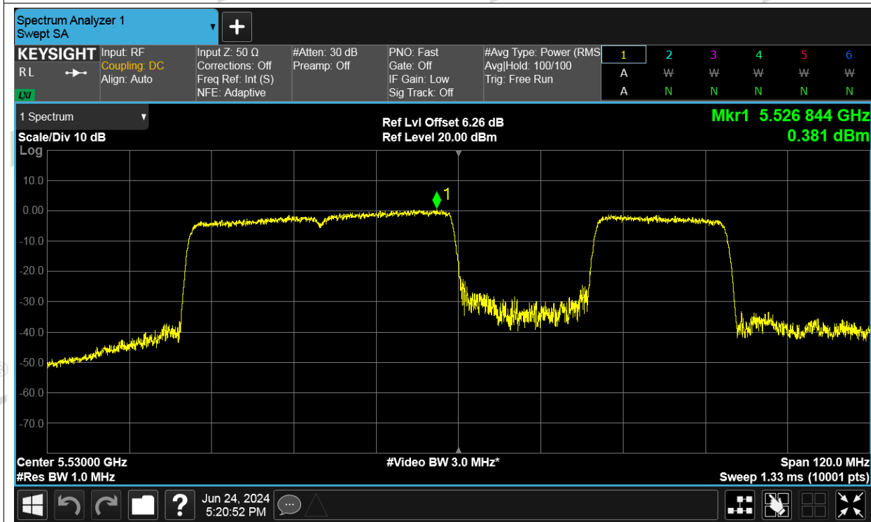
PSD NVNT be80 484+242-tone in a non-OFDMA MRU3 5530MHz Ant3
