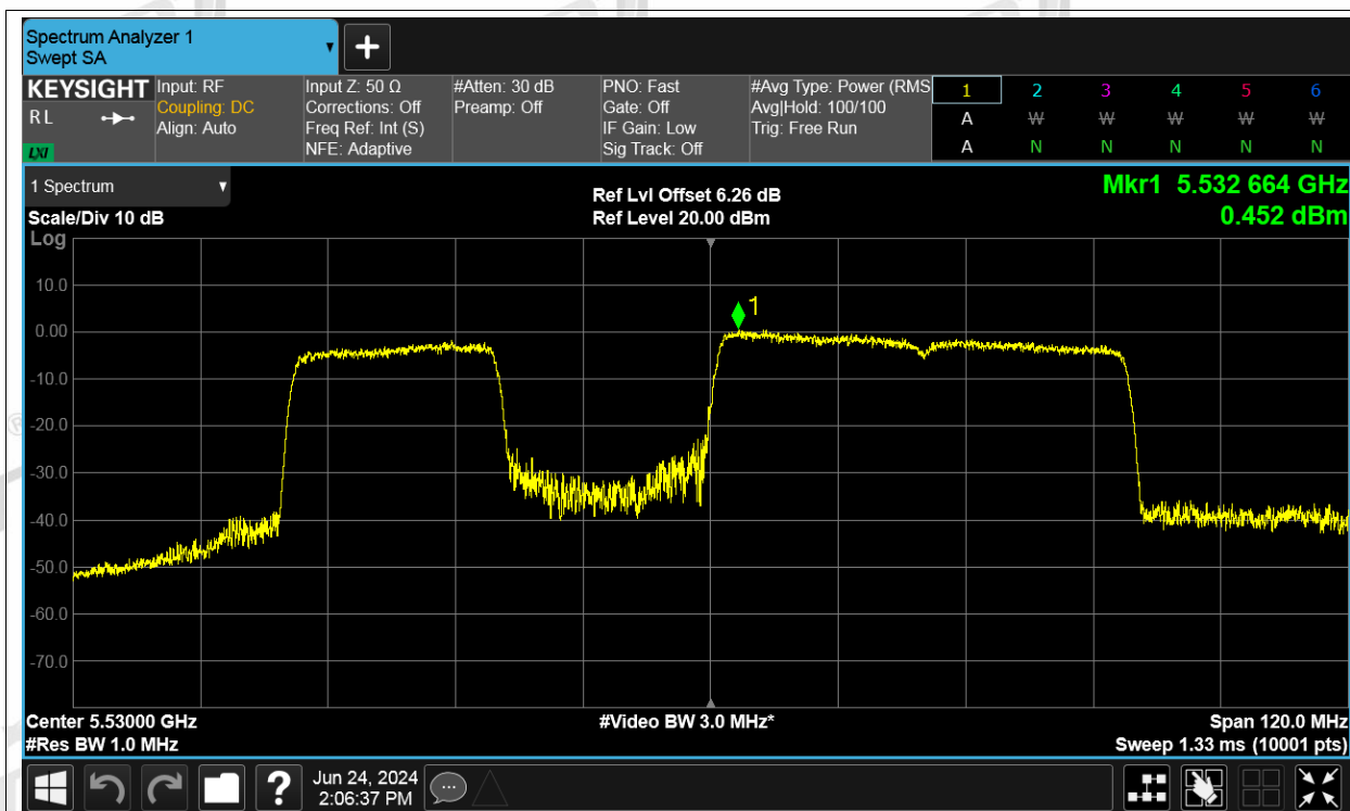
PSD NVNT be80 484+242-tone in a non-OFDMA MRU2 5530MHz Ant3
