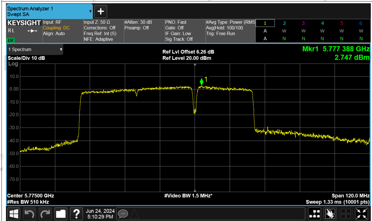
PSD NVNT be80 484+242-tone in a non-OFDMA MRU4 5775MHz Ant2
