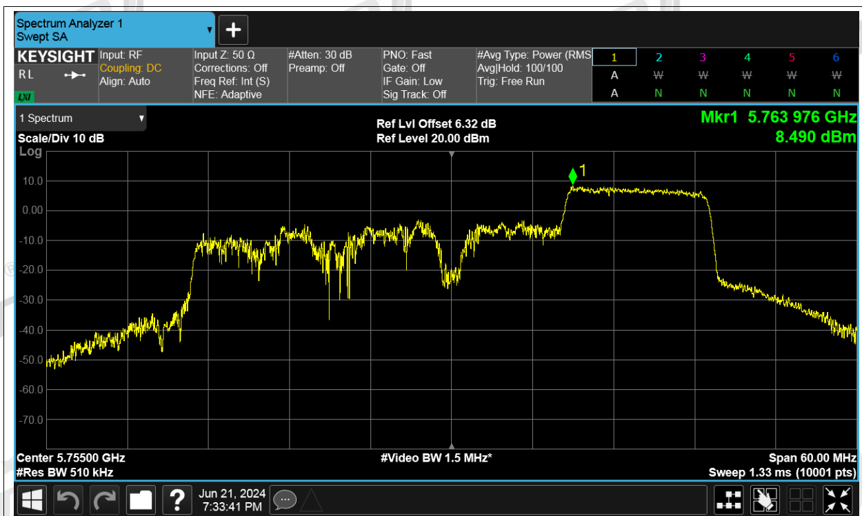
PSD NVNT be40 106+26RU Index 56+13 5755MHz Ant3
