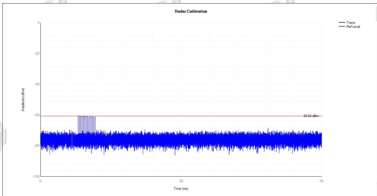
5530MHz DFS_FCC_T5000
