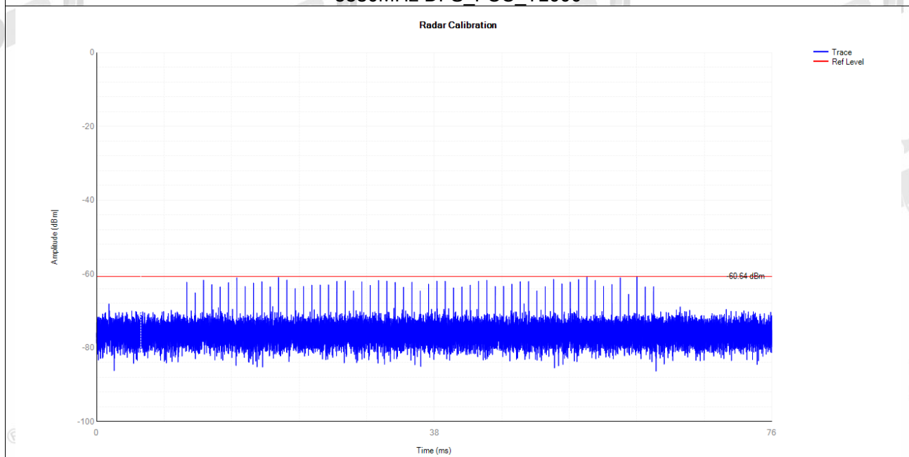
5530MHz DFS_FCC_T2000
