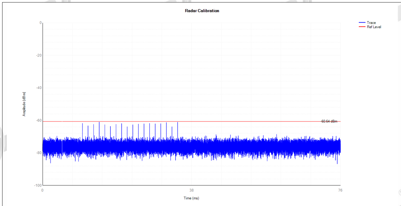
5530MHz DFS_FCC_T1000
