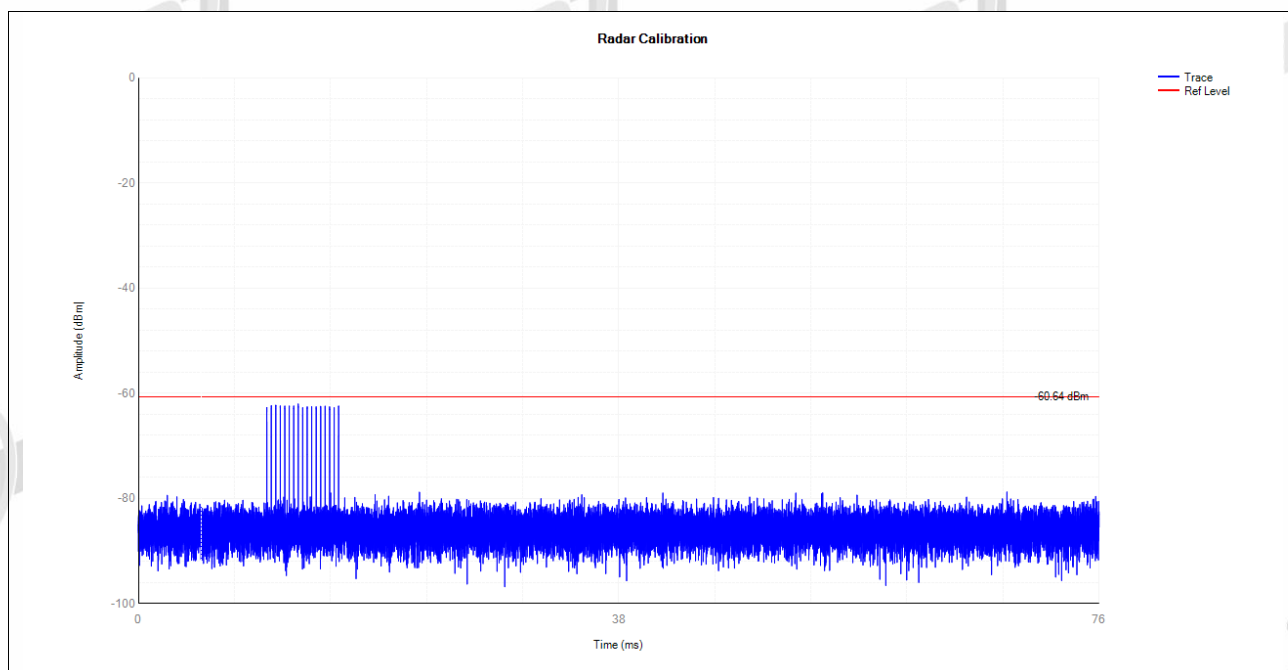
5570MHz DFS_FCC_T4000
