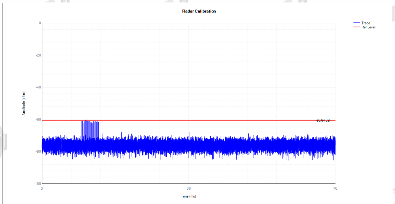
5530MHz DFS_FCC_T3000
