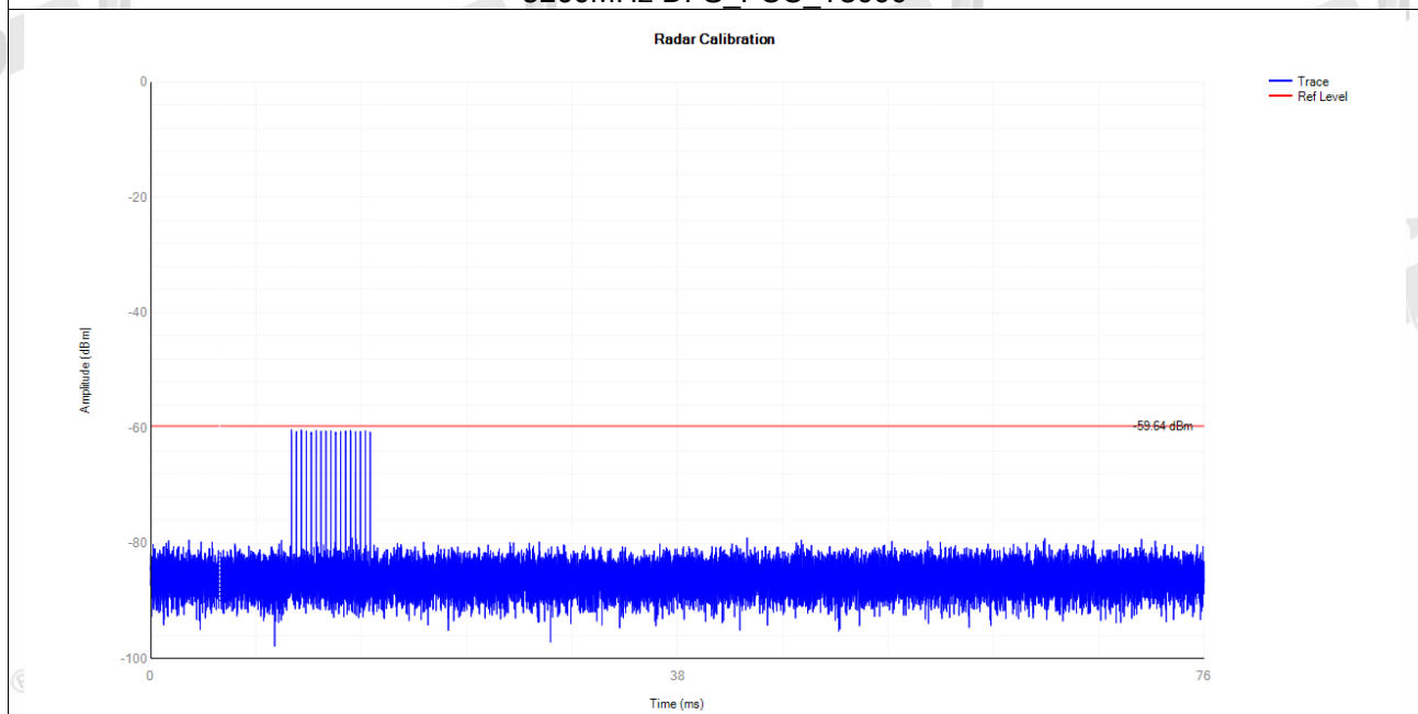
5260MHz DFS_FCC_T4000
