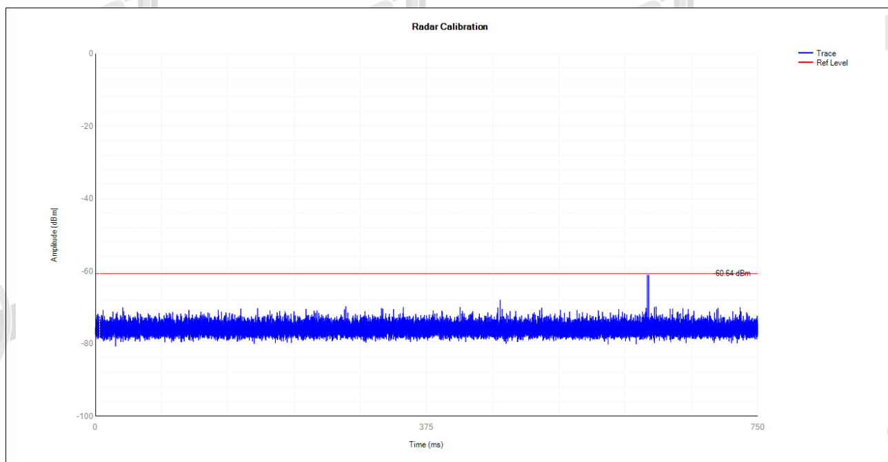
5510MHz DFS_FCC_T6000
