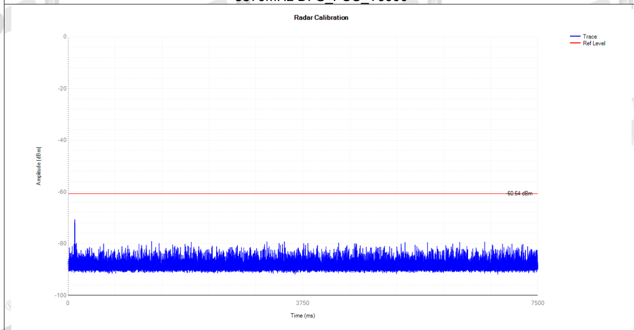
5260MHz DFS_FCC_T0
