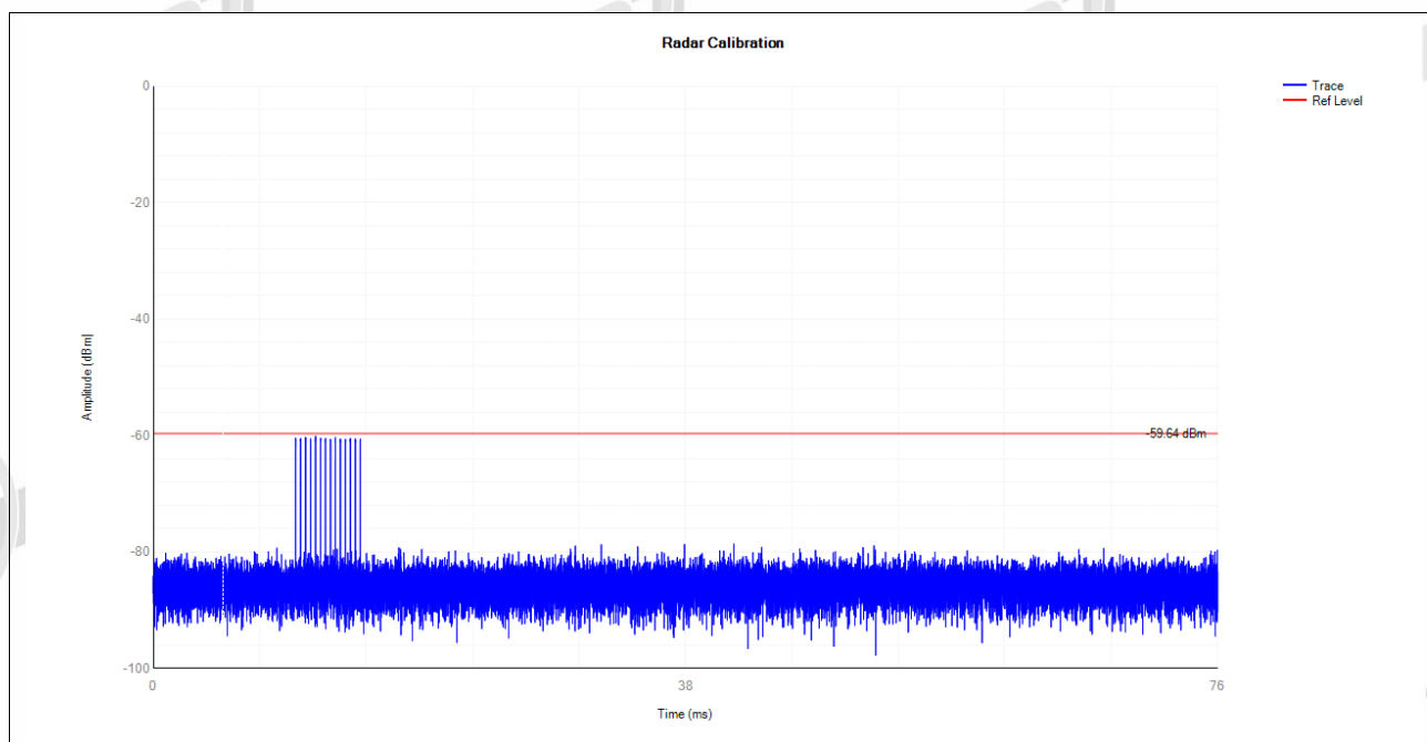
5260MHz DFS_FCC_T5000
