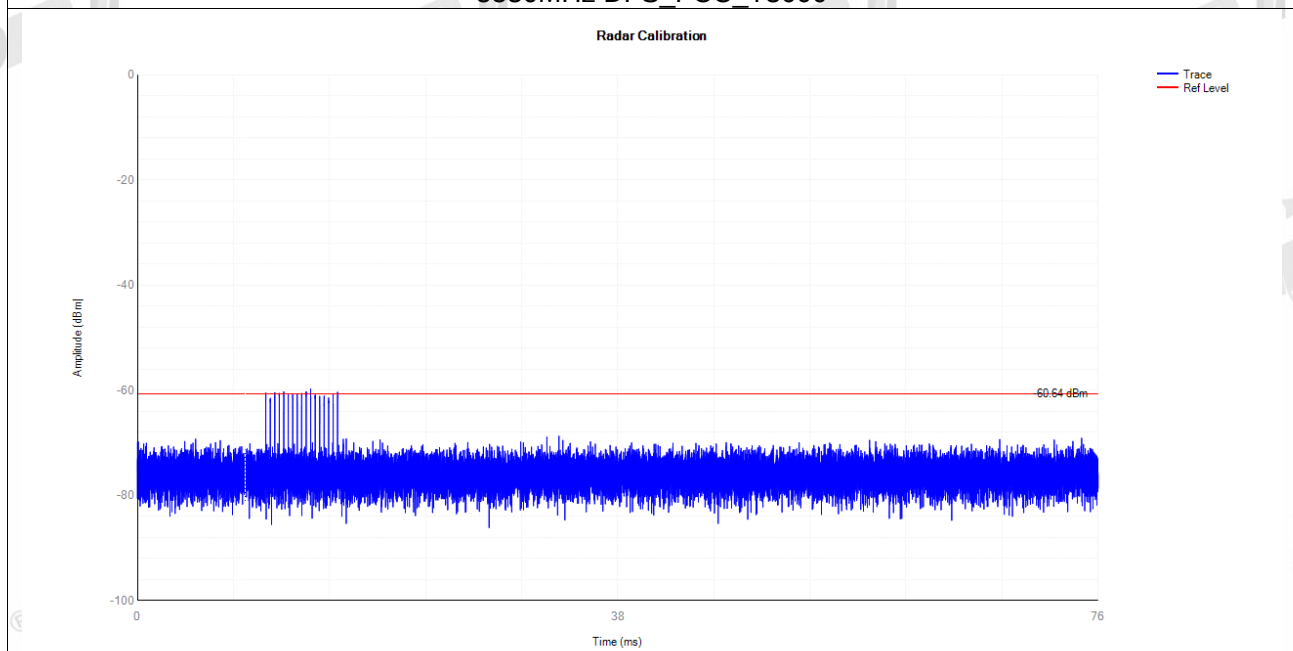
5530MHz DFS_FCC_T4000
