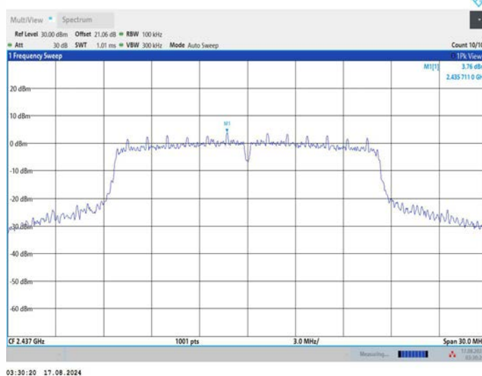
11G_Ant1_2437_0~Reference
