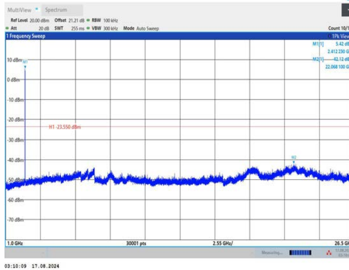
11B_Ant2_2412_0~Reference
