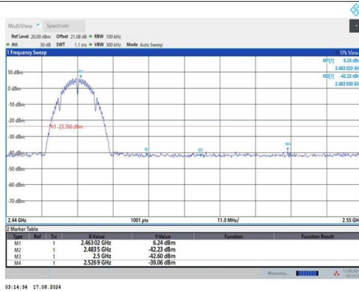
11B_Ant2_High_2462
