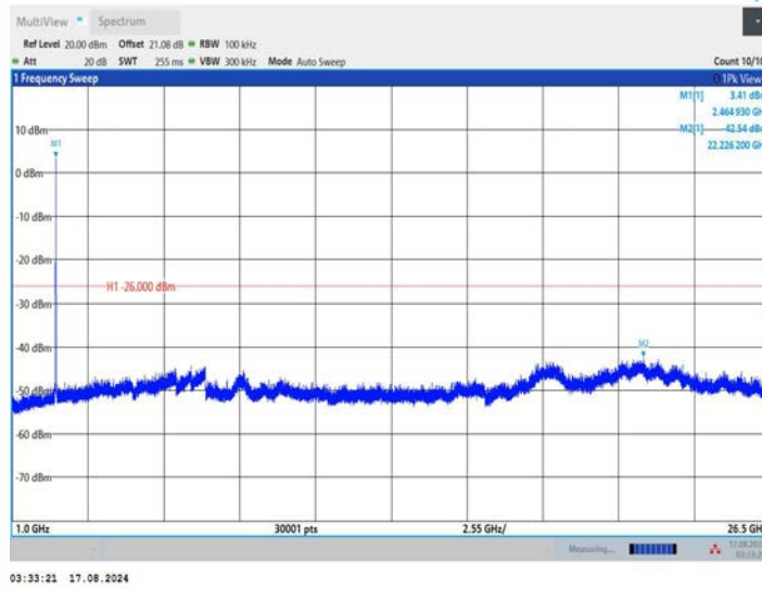
11G_Ant2_2462_0~Reference
