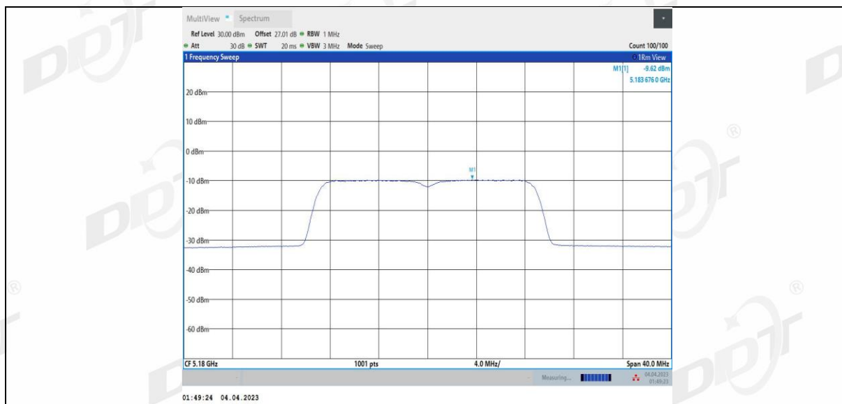
11AC20MIMO_Ant4_5180
