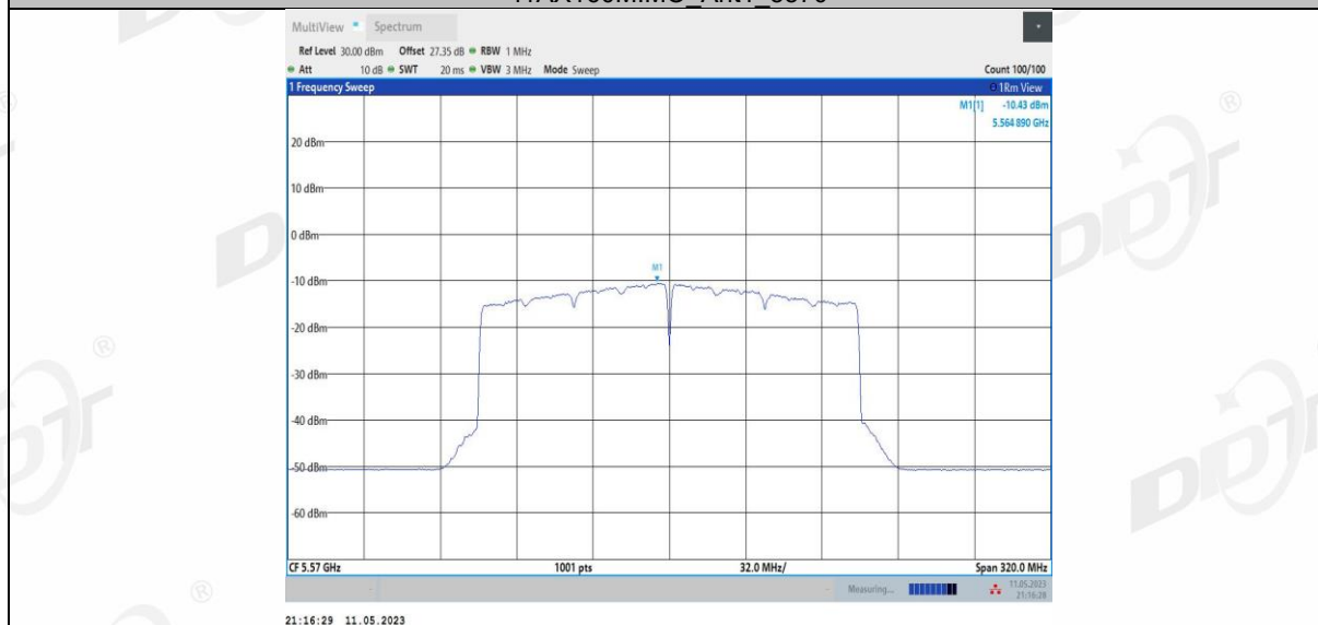
11AX160MIMO Ant2 5570
