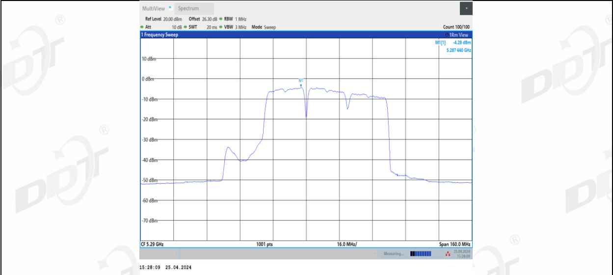
11BE80MIMO Ant2 5290 484+242 Non-OFDMA 2
