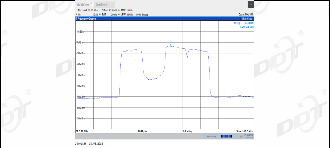
11BE80MIMO Ant2 5290 484+242 Non-OFDMA 3
