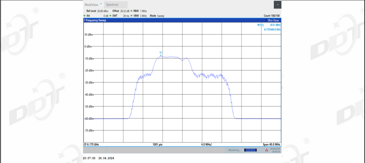
11BE20MIMO Ant1_6175_52+26_3
