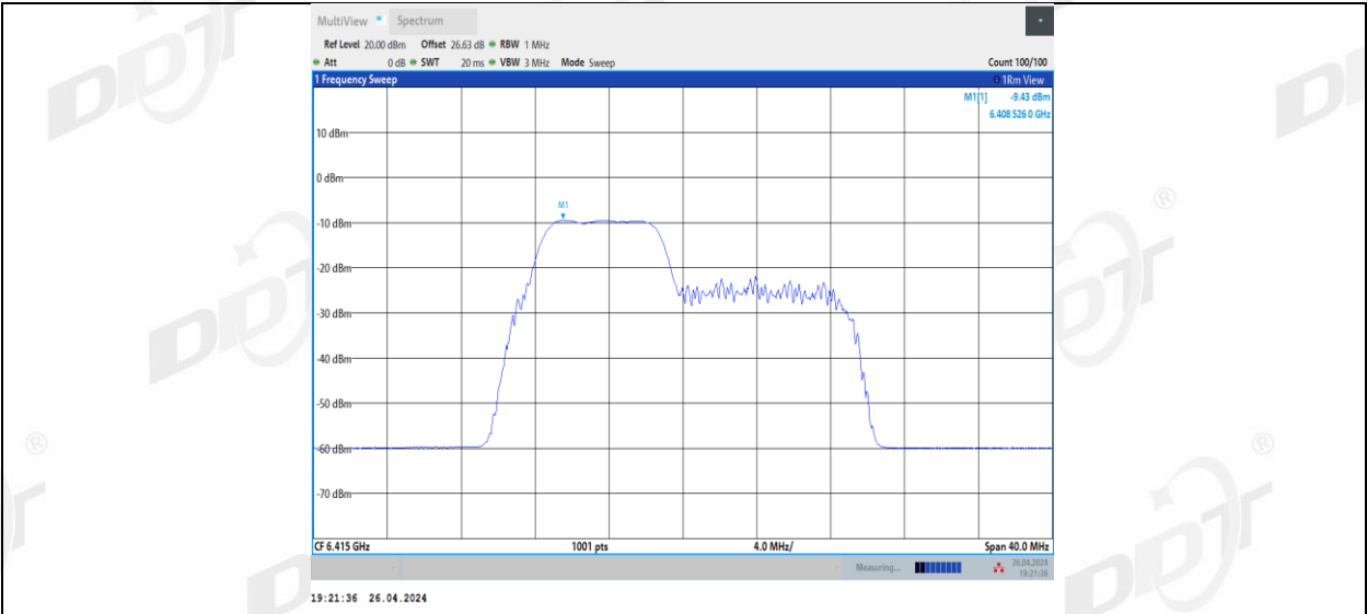
11BE20MIMO Ant1_6415_52+26_2
