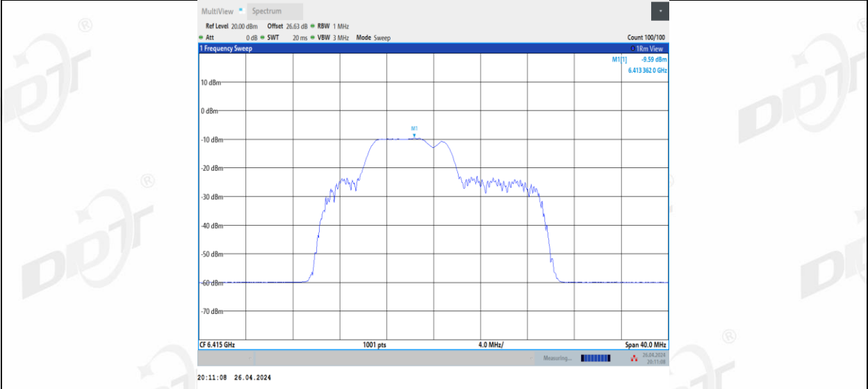
11BE20MIMO Ant1_6415_52+26_3
