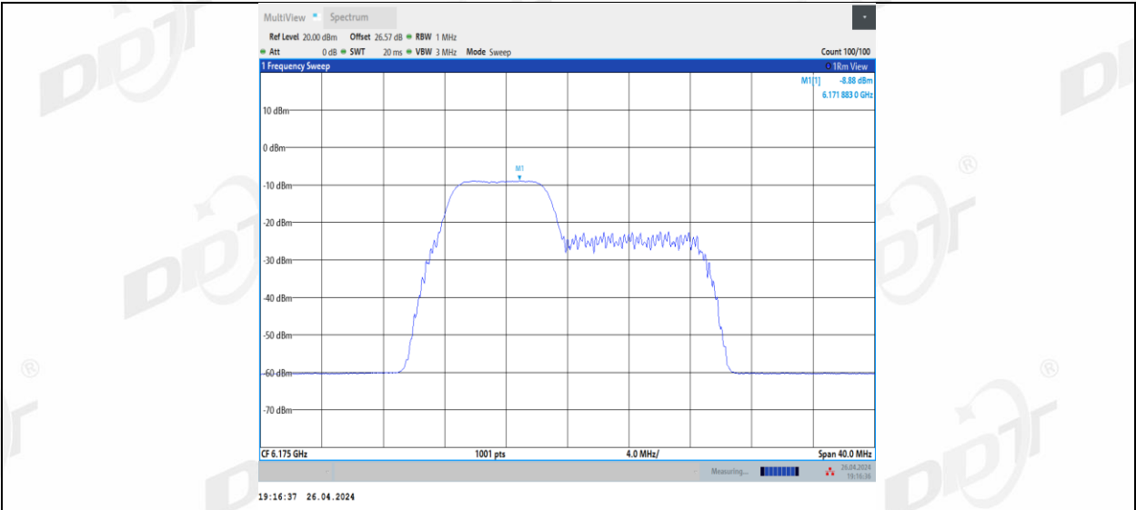
11BE20MIMO Ant1_6175_52+26_2
