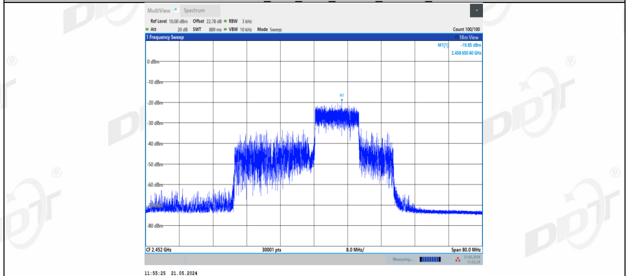
11BE40MIMO_Ant1_2452_106+26_OFDMA_4
