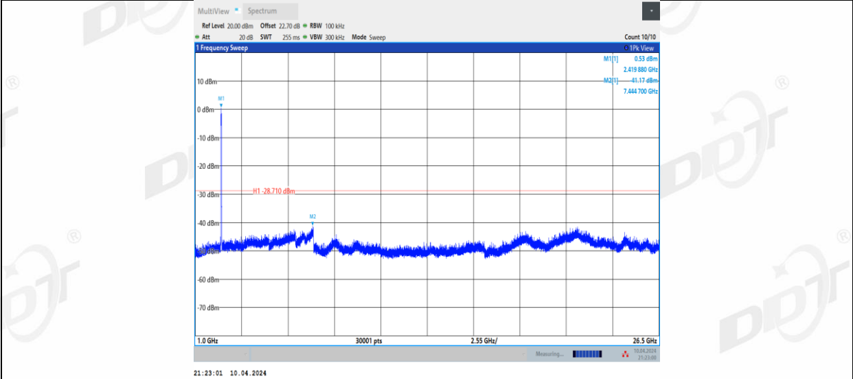
11BE40MIMO_Ant1_2437_0~Reference
