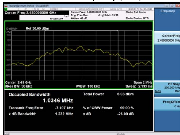
BLE 1M Carrier frequency (MHz): 2480
