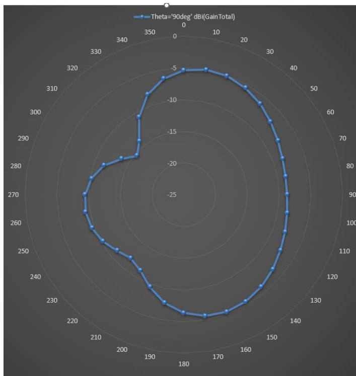
ZY theta90 phi0-360
