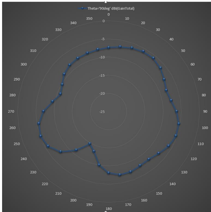
ZY theta90 phi0-360
