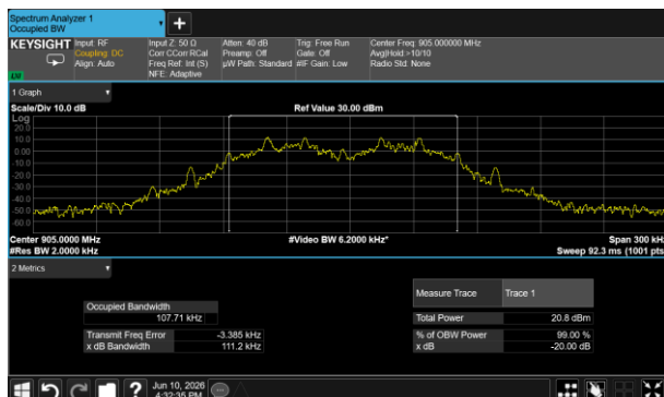
20dB Bandwidth plot on channel 103
