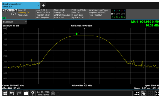
Peak output Power plot on channel 103
