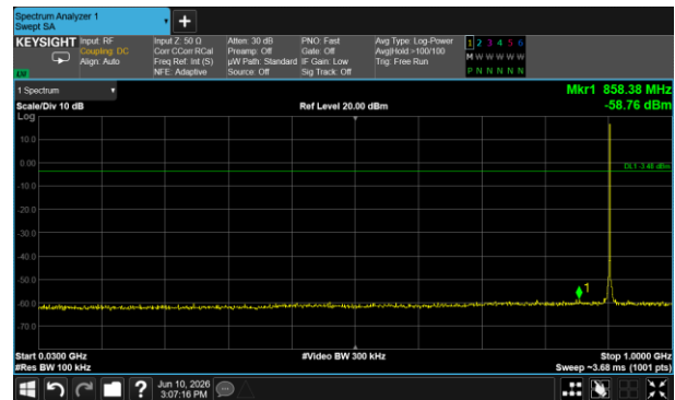
GFSK on channel 01
