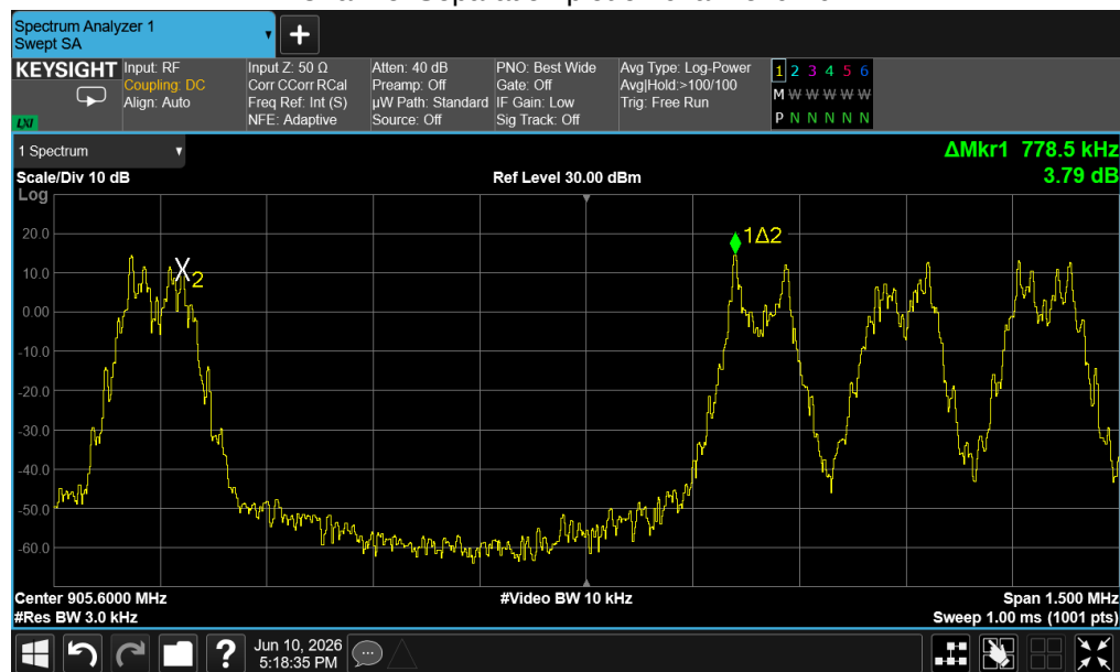
Channel Separation plot on channel 01-02
