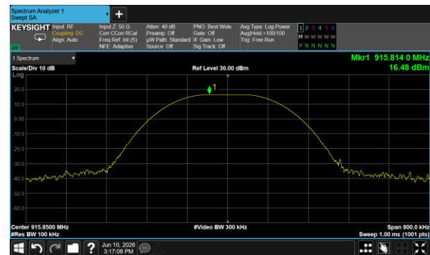
Peak output Power plot on channel 52
