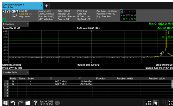
GFSK: Band Edge-Low Channel (Hopping Mode)
