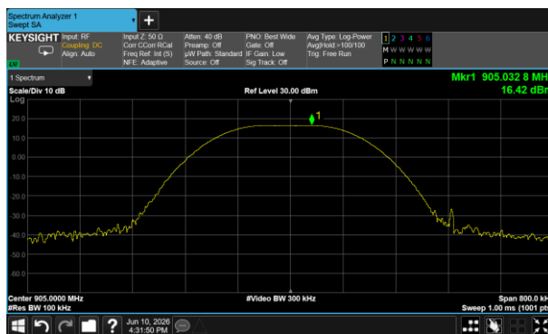
Peak output Power plot on channel 01
