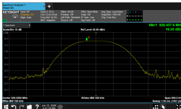
Peak output Power plot on channel 103
