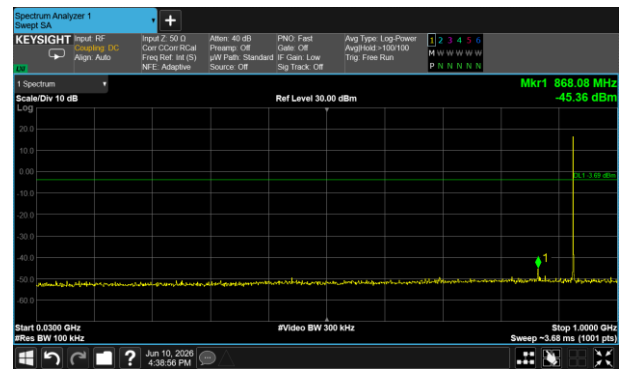
GFSK on channel 103
