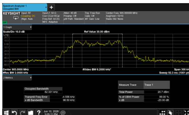
20dB Bandwidth plot on channel 01
