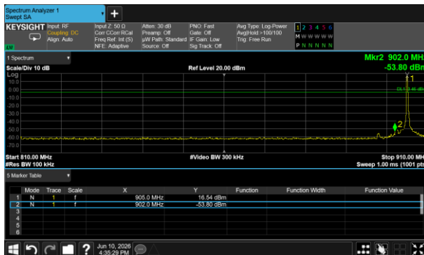
GFSK: Band Edge-Low Channel (Hopping Mode)
