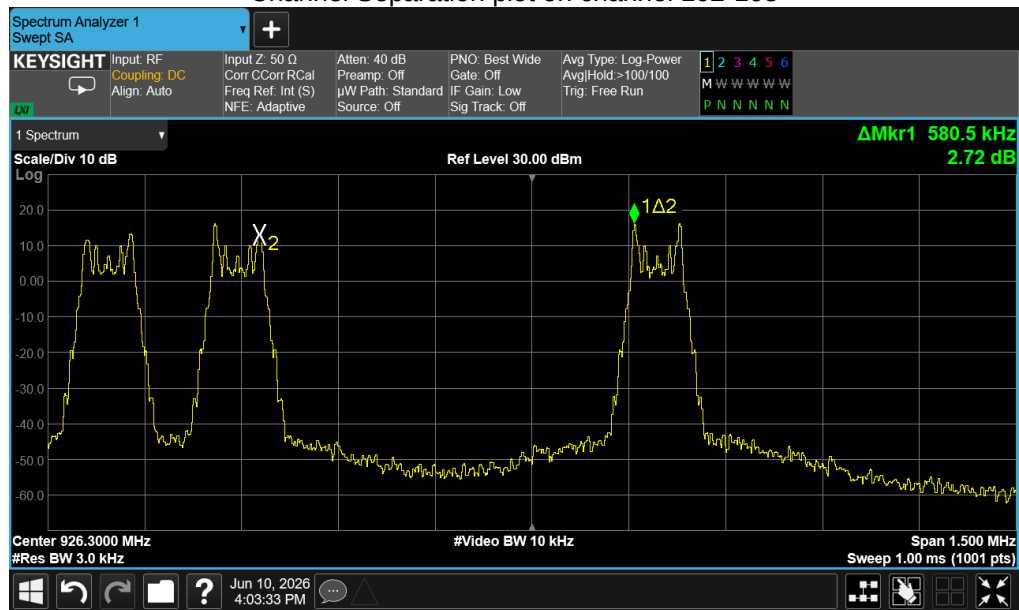
Channel Separation plot on channel 102-103
