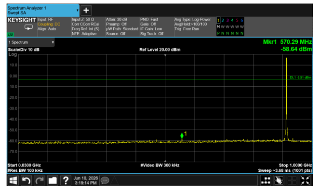
GFSK on channel 52
