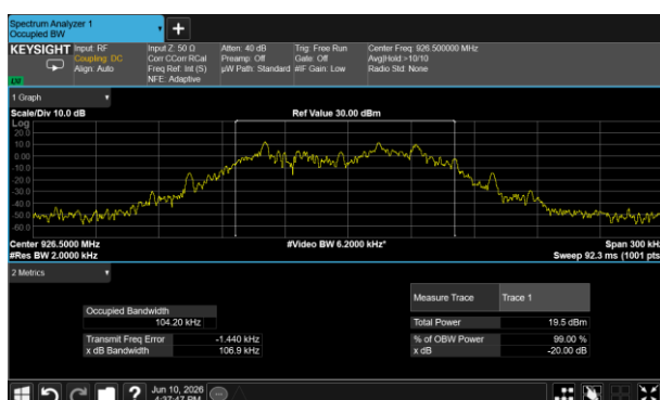
20dB Bandwidth plot on channel 103
