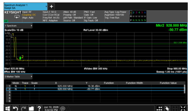
GFSK: Band Edge-High Channel (Hopping Mode)
