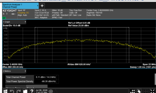
Conducted AVG output power IEEE 802.11b Channel 11 Antenna 0
