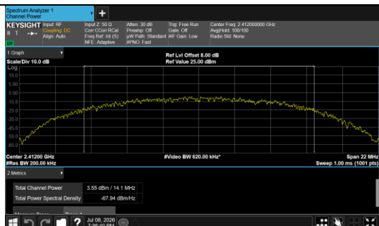
Conducted AVG output power IEEE 802.11b Channel 1 Antenna 0
