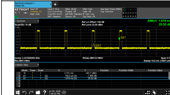
IEEE 802.11g 20MHz Channel 6
