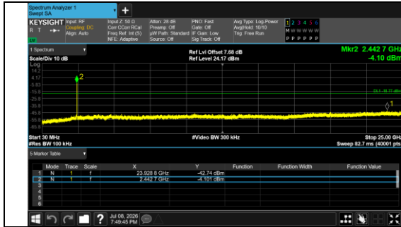
30.0 MHz - 25000.0 MHz IEEE 802.11g Channel 6 20MHz Antenna 0
