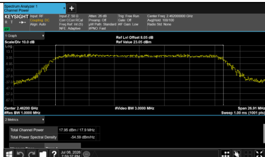
Conducted Output Power IEEE 802.11n 20 Channel 11 Antenna 0
