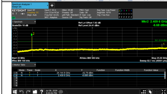
30.0 MHz - 25000.0 MHz IEEE 802.11n Channel 3 40MHz Antenna 0
