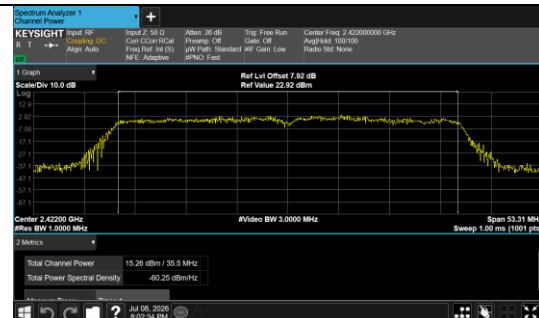
Conducted Output Power IEEE 802.11n 40 Channel 3 Antenna 0
