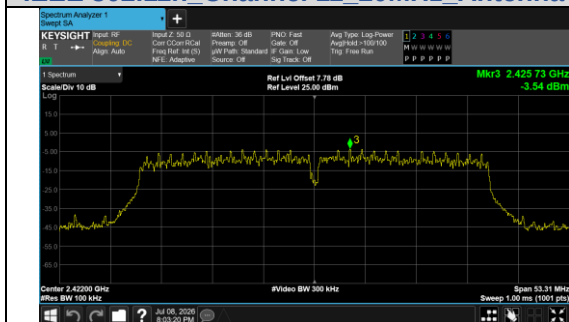
In-Band Reference Level IEEE 802.11n Channel 3 40MHz Antenna 0
