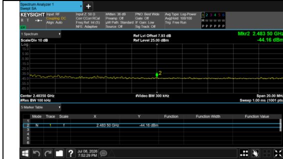
Out Of Band Emission IEEE 802.11g Channel 11 20MHz Antenna 0
