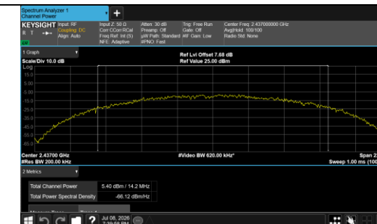
Conducted AVG output power IEEE 802.11b Channel 6 Antenna 0
