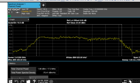
Conducted AVG output power IEEE 802.11g Channel 1 Antenna 0
