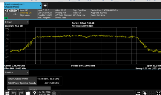
Conducted Output Power IEEE 802.11n 40 Channel 9 Antenna 0
