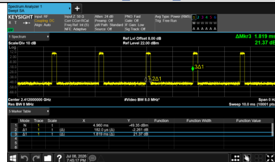
IEEE 802.11g 20MHz Channel 1
