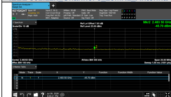
Out Of Band Emission IEEE 802.11n Channel 11 20MHz Antenna 0
