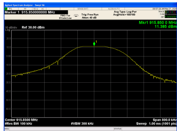
Peak output Power plot on channel 52
