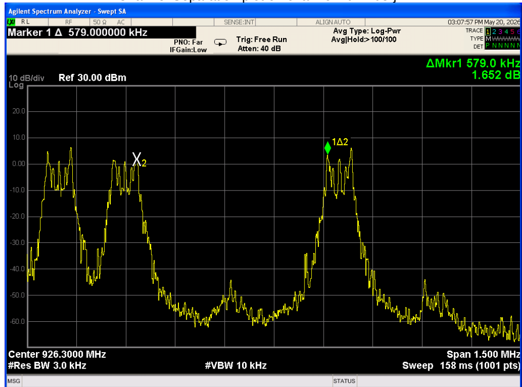
Channel Separation plot on channel 102-103-jwl
