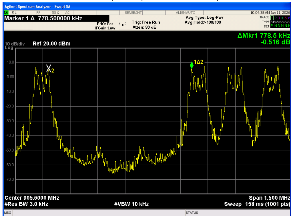
Channel Separation plot on channel 01-02-jwl
