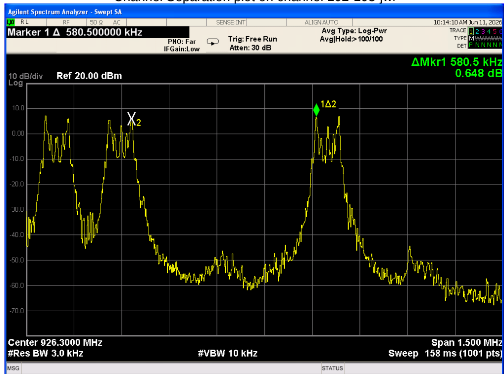
Channel Separation plot on channel 102-103-jwl
