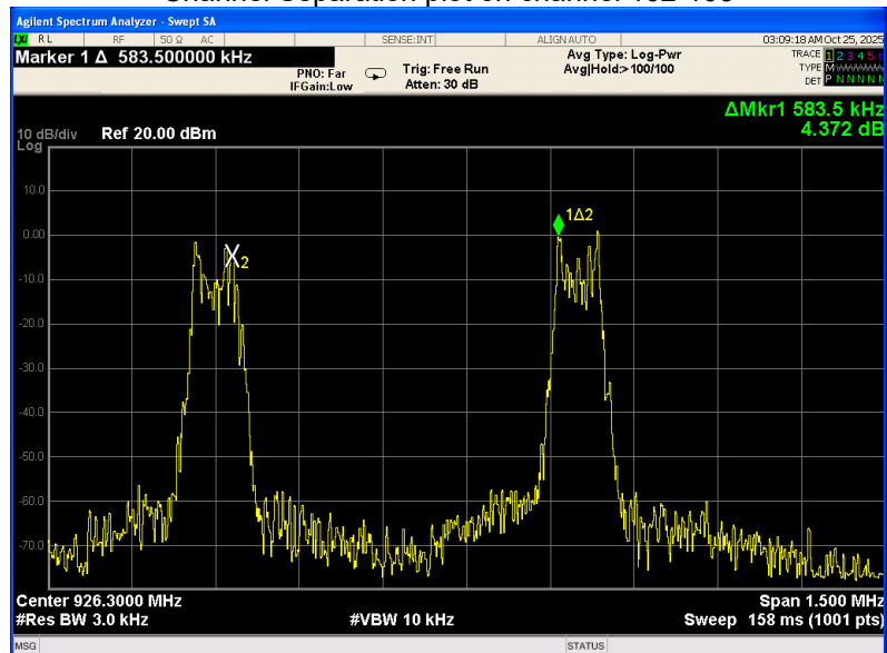
Channel Separation plot on channel 102-103
