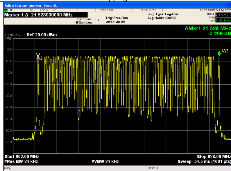
Number of Hopping Channel Plot
