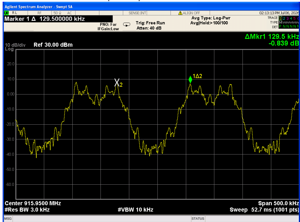
Channel Separation plot on channel 52-53-WNG
