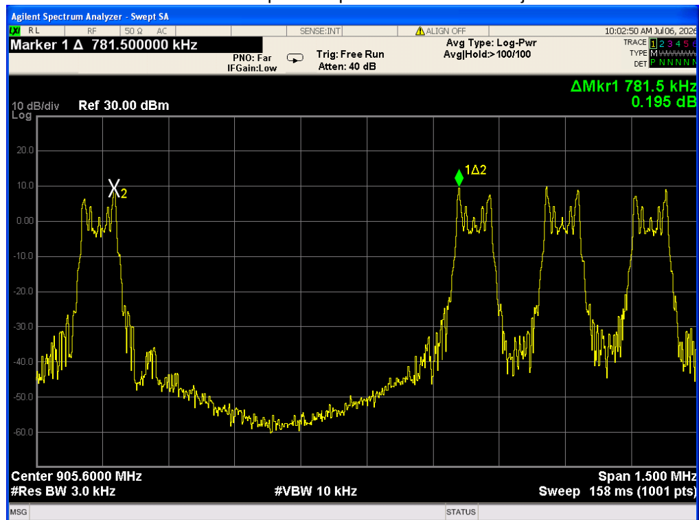
Channel Separation plot on channel 01-02-jwl
