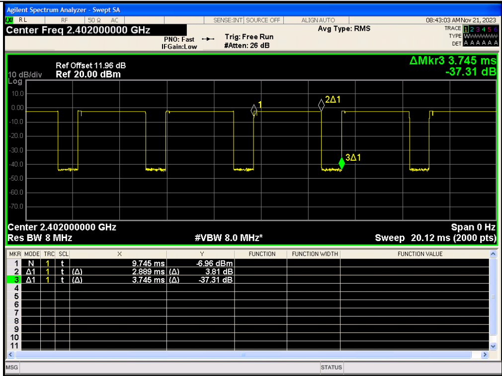
8DPSK(3-DH5)_Channel 0
