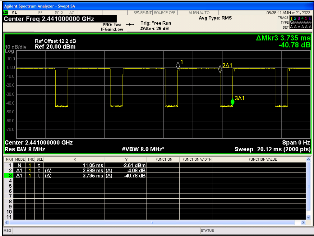
π/4DQPSK(2-DH5)_Channel 39
