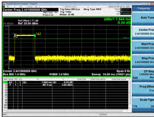
Burst(2DH3)
