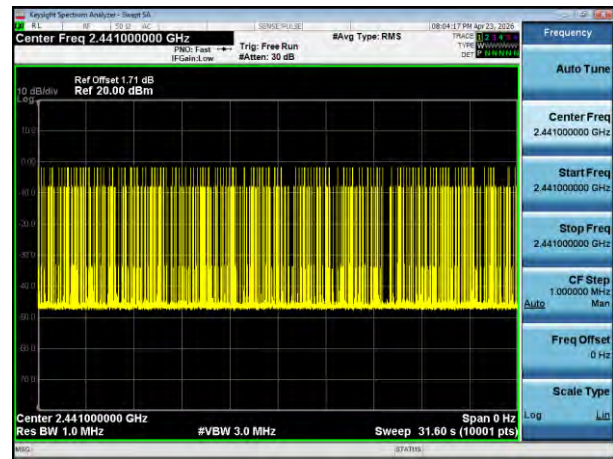
Accumulate(2DH3)
