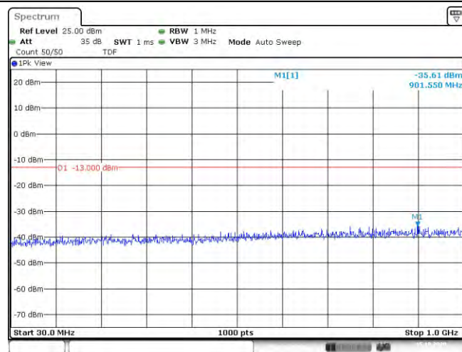
Band25-3MHz-16QAM-26675-1RB#0-Range1:30~1000MHz
