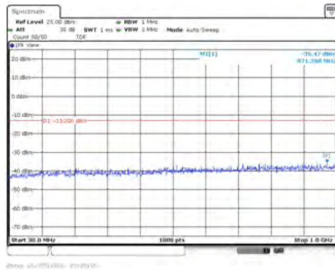
Band25-3MHz-QPSK-26365-1RB#0-Range1:30~1000MHz
