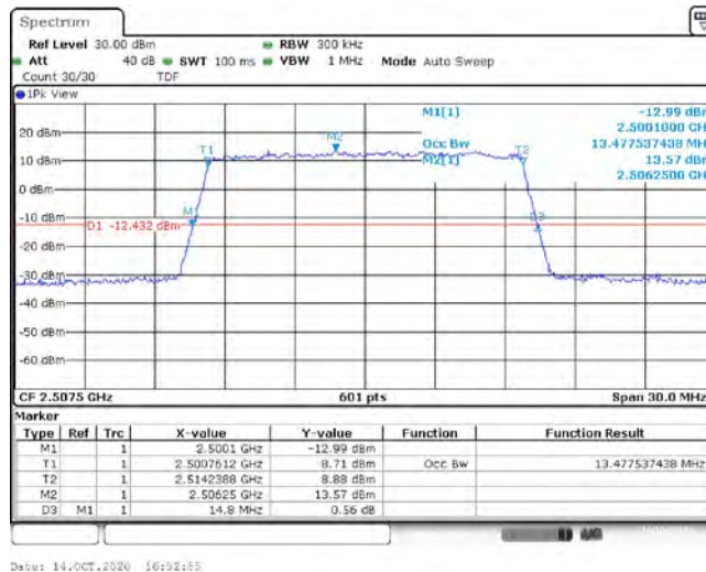
Band7-15MHz-16QAM-21100-75RB#0-13.478
