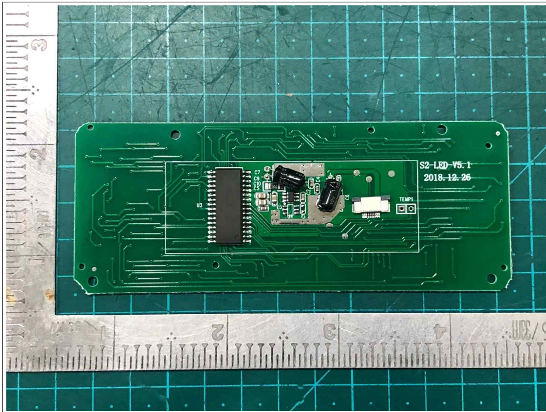
View of PCB 2 (Bottom)
