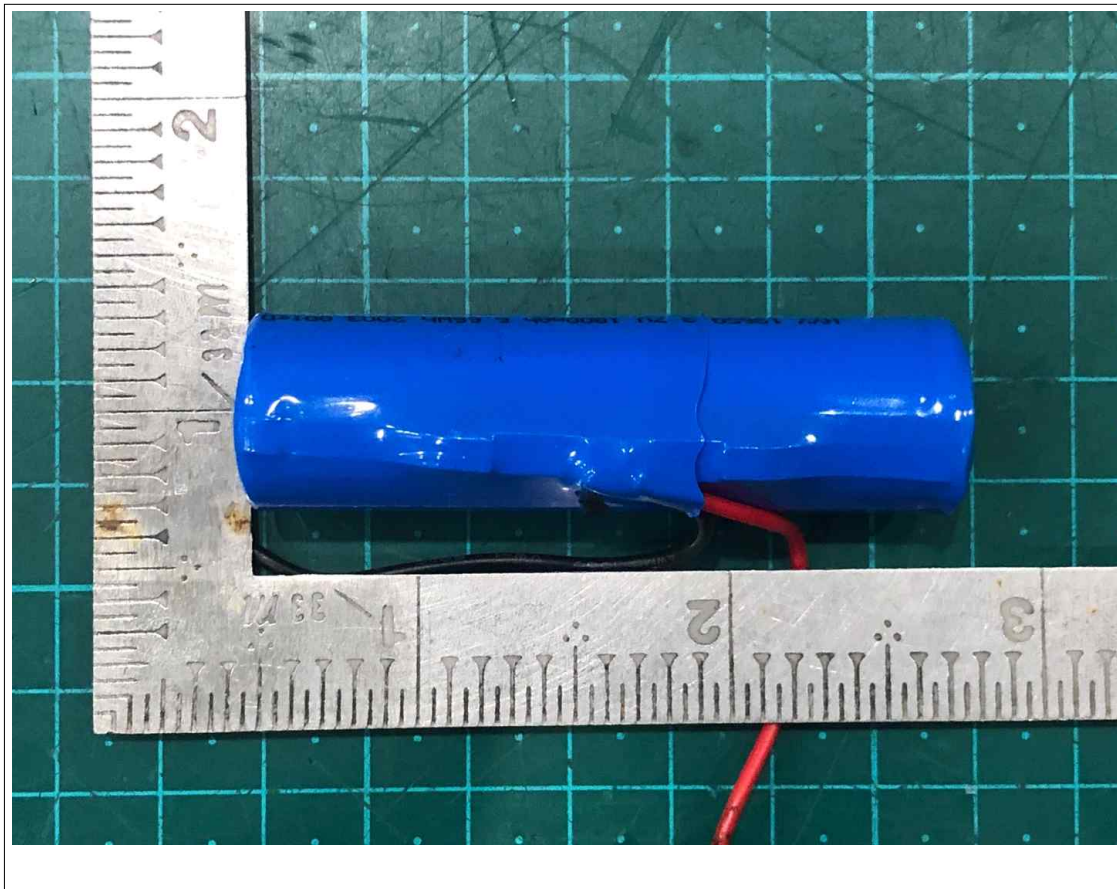
View of Battery (Bottom)
