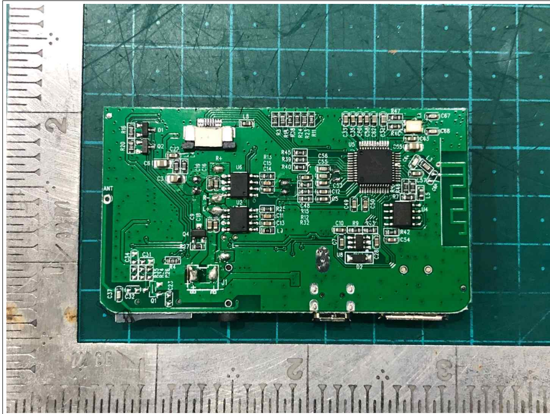
View of PCB 1 (Bottom)
