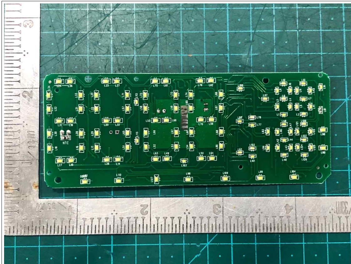
View of PCB 2 (Top)
