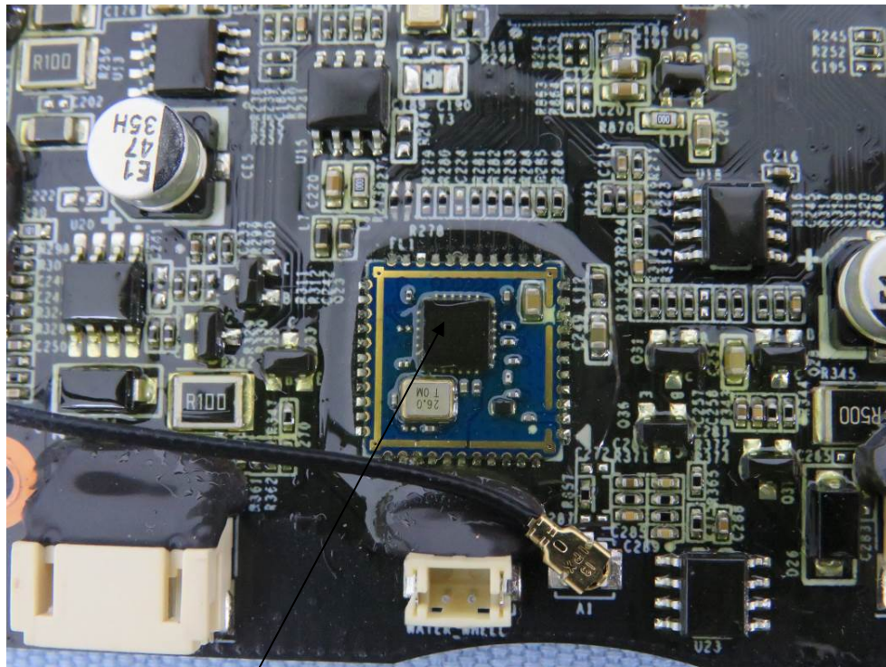
RF Chip
