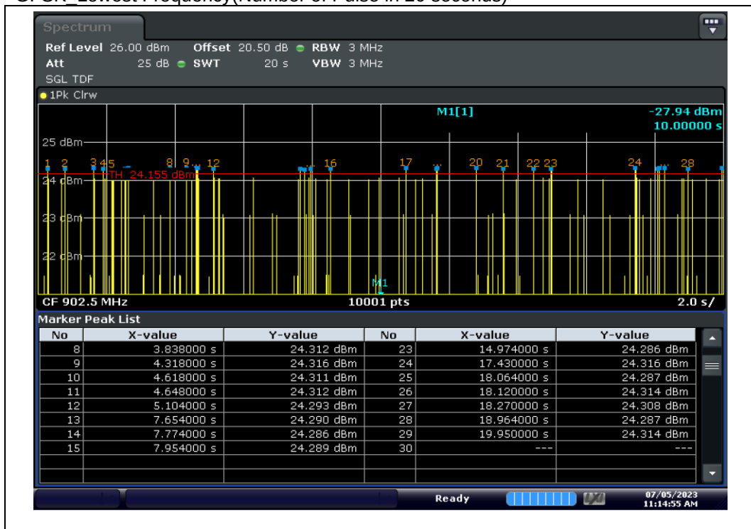
GFSK Lowest Frequency(Number of Pulse in 20 seconds)
