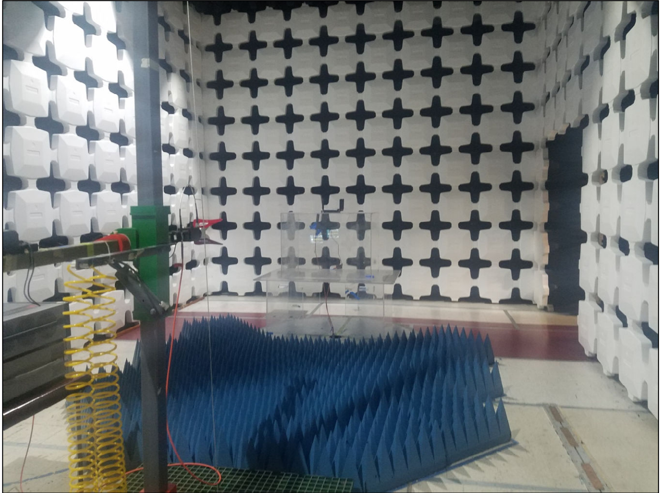
Radiated Spurious Emissions, 1GHz – 18GHz, Test Setup
