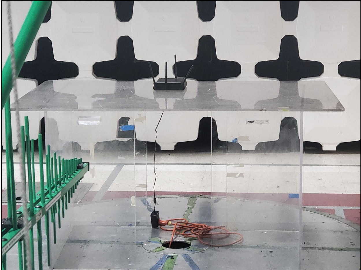
Radiated Spurious Emissions, 1GHz – 18GHz, Test Setup
