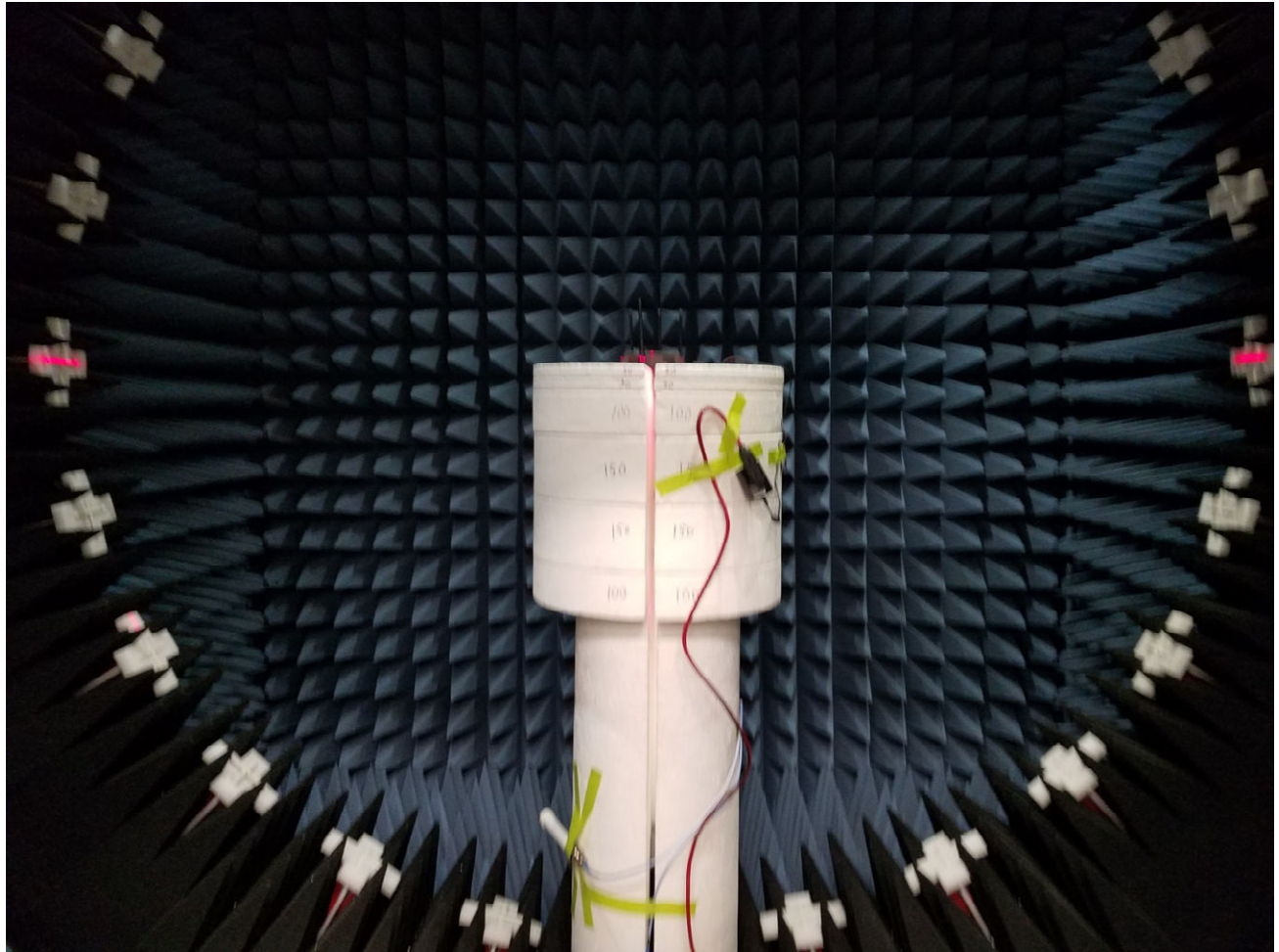
OTA EIRP Test Setup View 2
