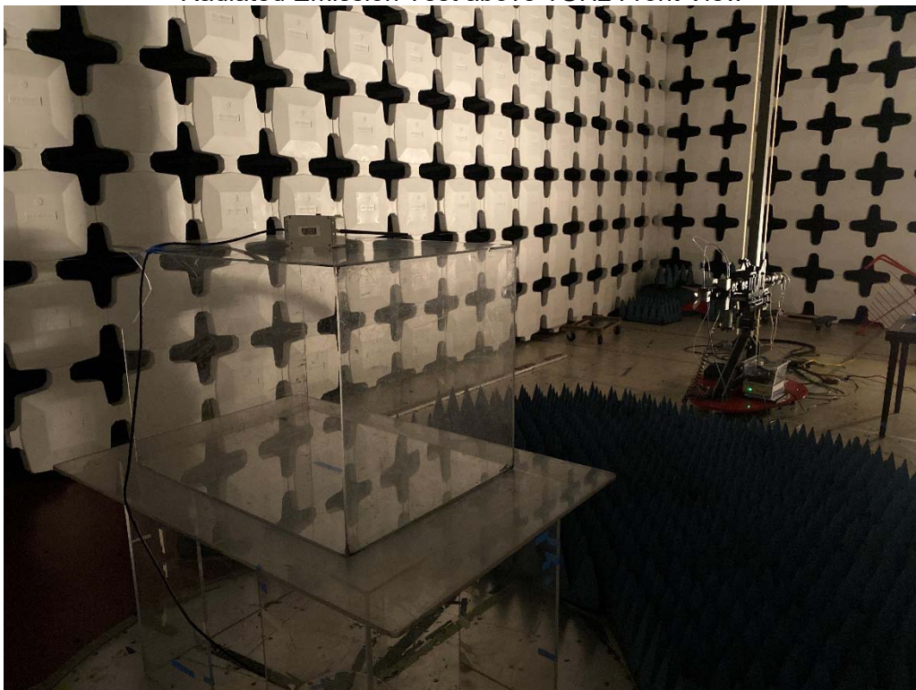
Radiated Emission Test above 1GHz Rear View
