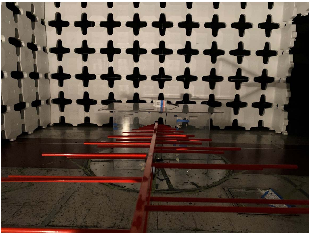
Radiated Emission Test below 1GHz Front View
