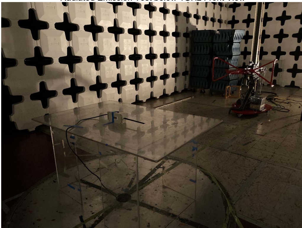
Radiated Emission Test below 1GHz Rear View
