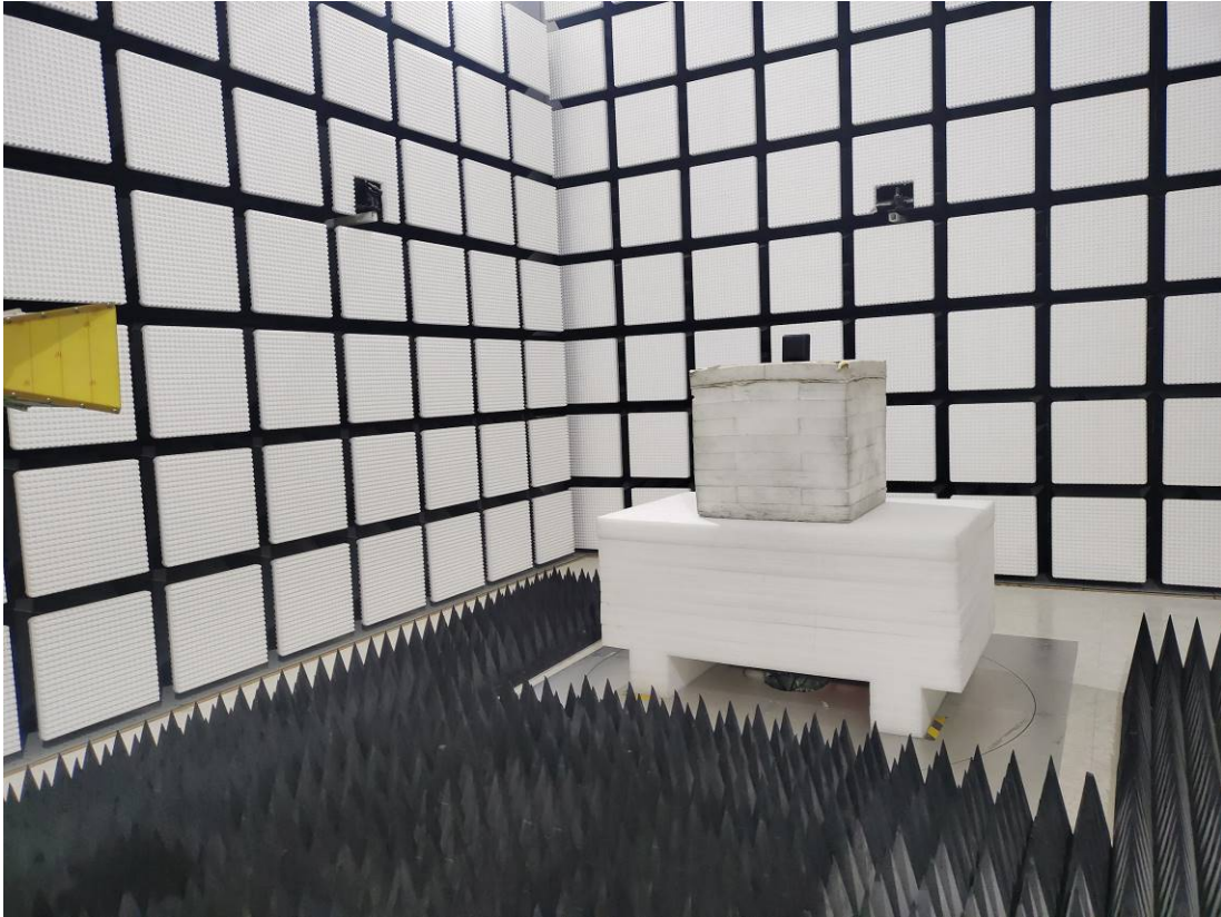
Radiated Emission Above 18G - 26.5GHz View
