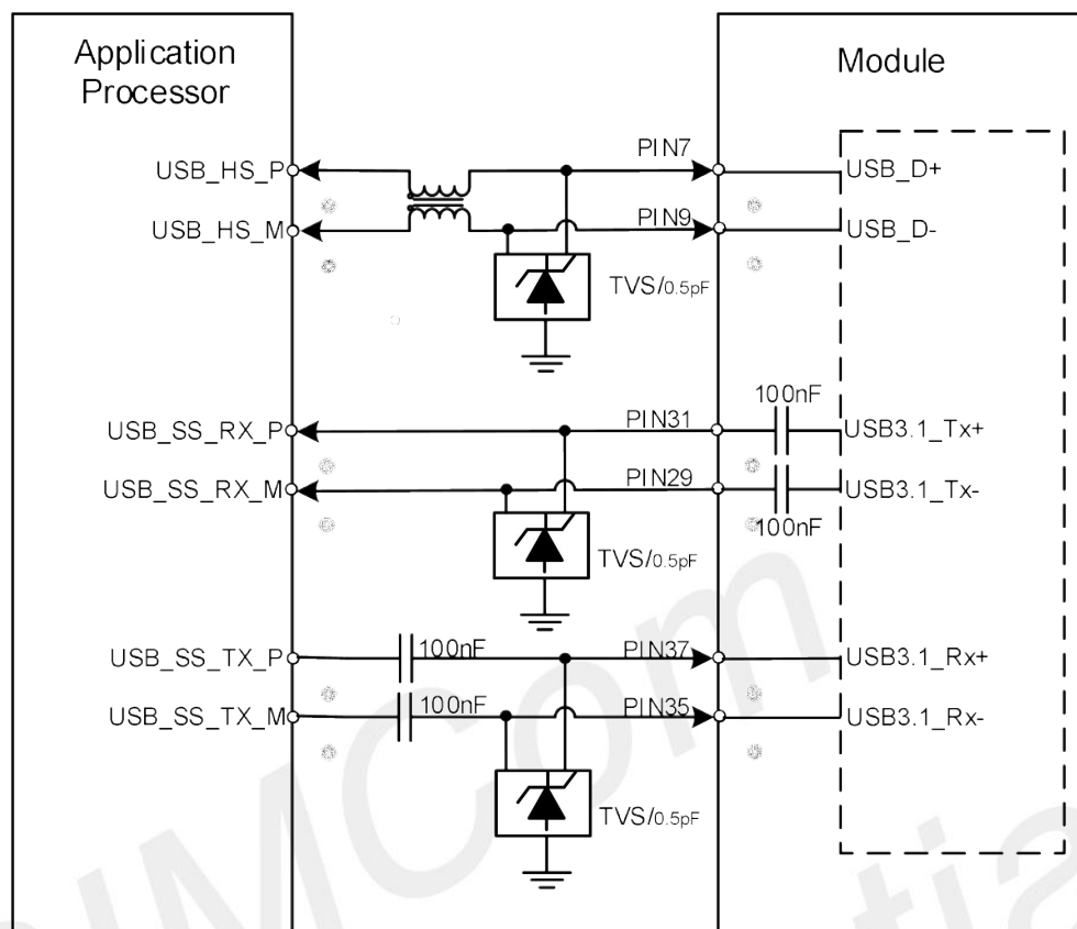
Figure 20: USB reference circuit
