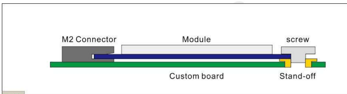
Figure 33: Equipment diagram
