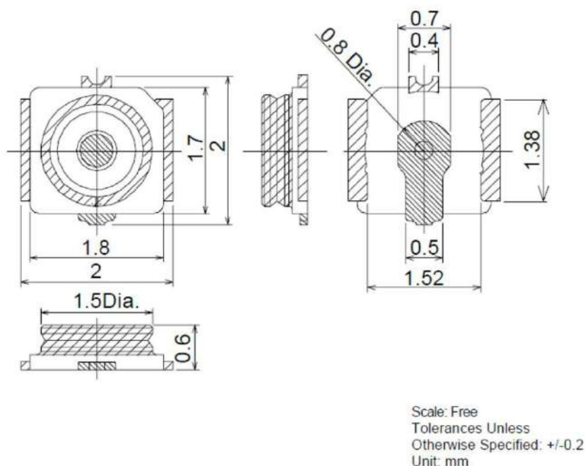
Figure 32: RF connector
