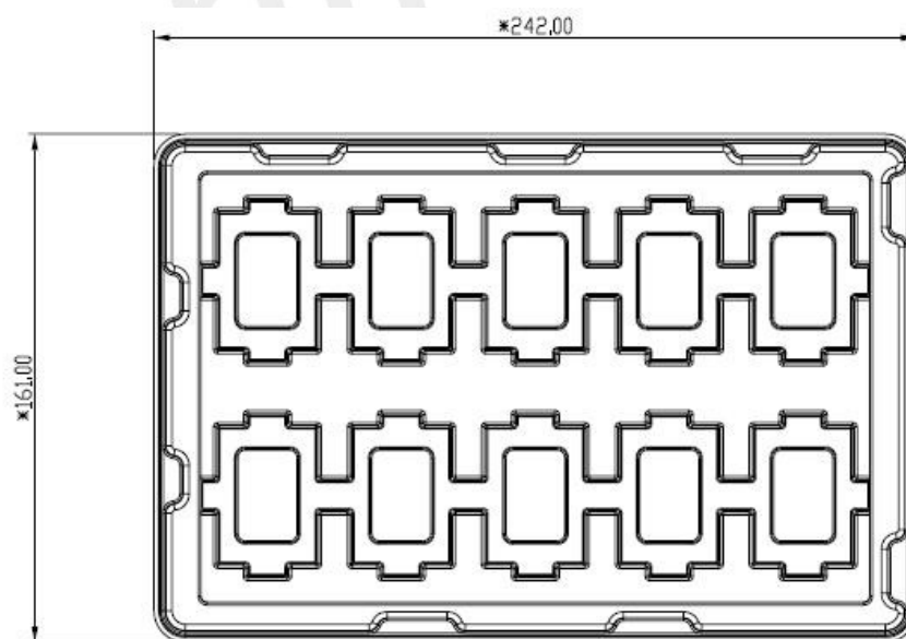
Figure 36: Tray drawing
