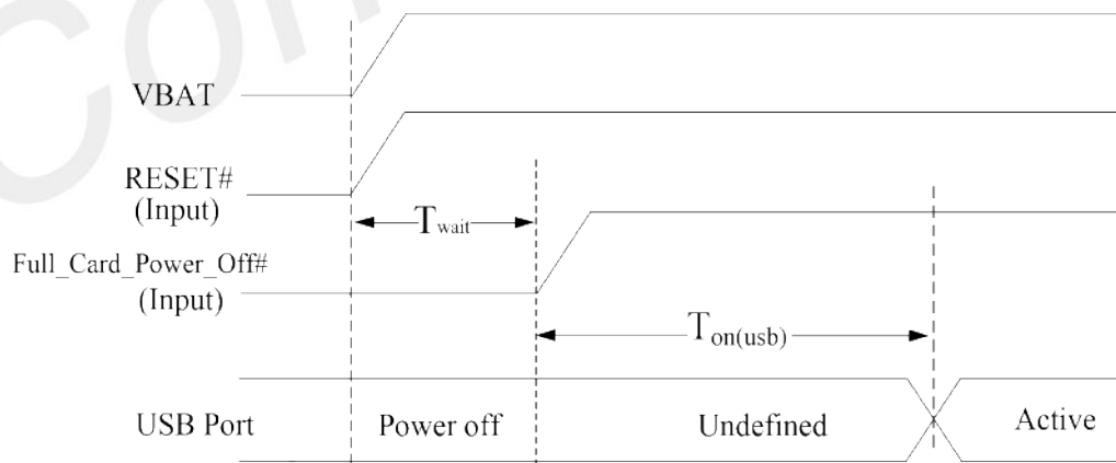
Figure 11: Power on timing sequence
