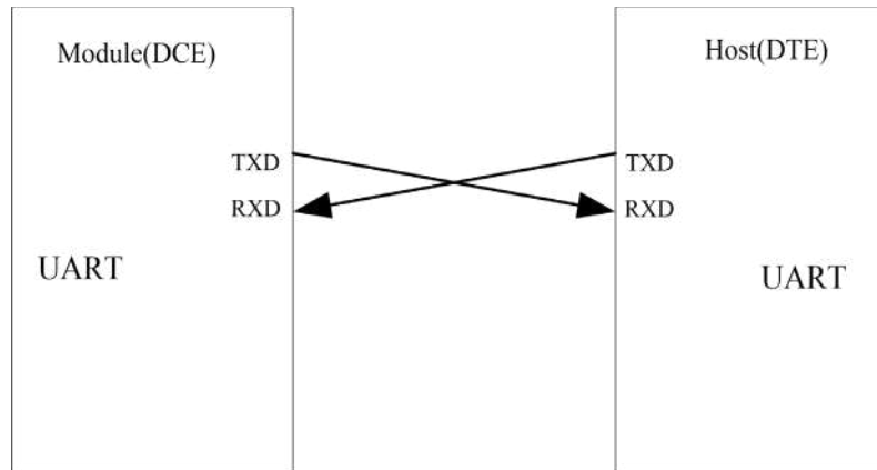
Figure 14: UART modem
