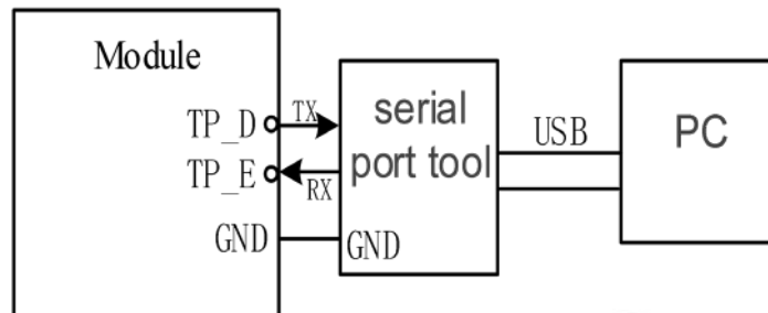
Figure 31: UART LOG
