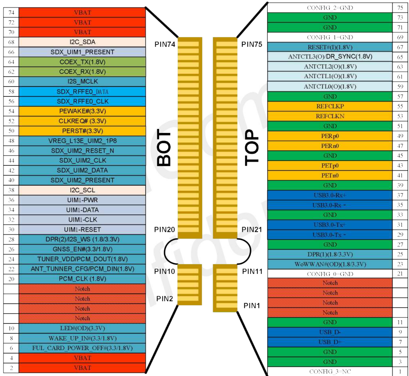
Figure 3: Pin assignment
