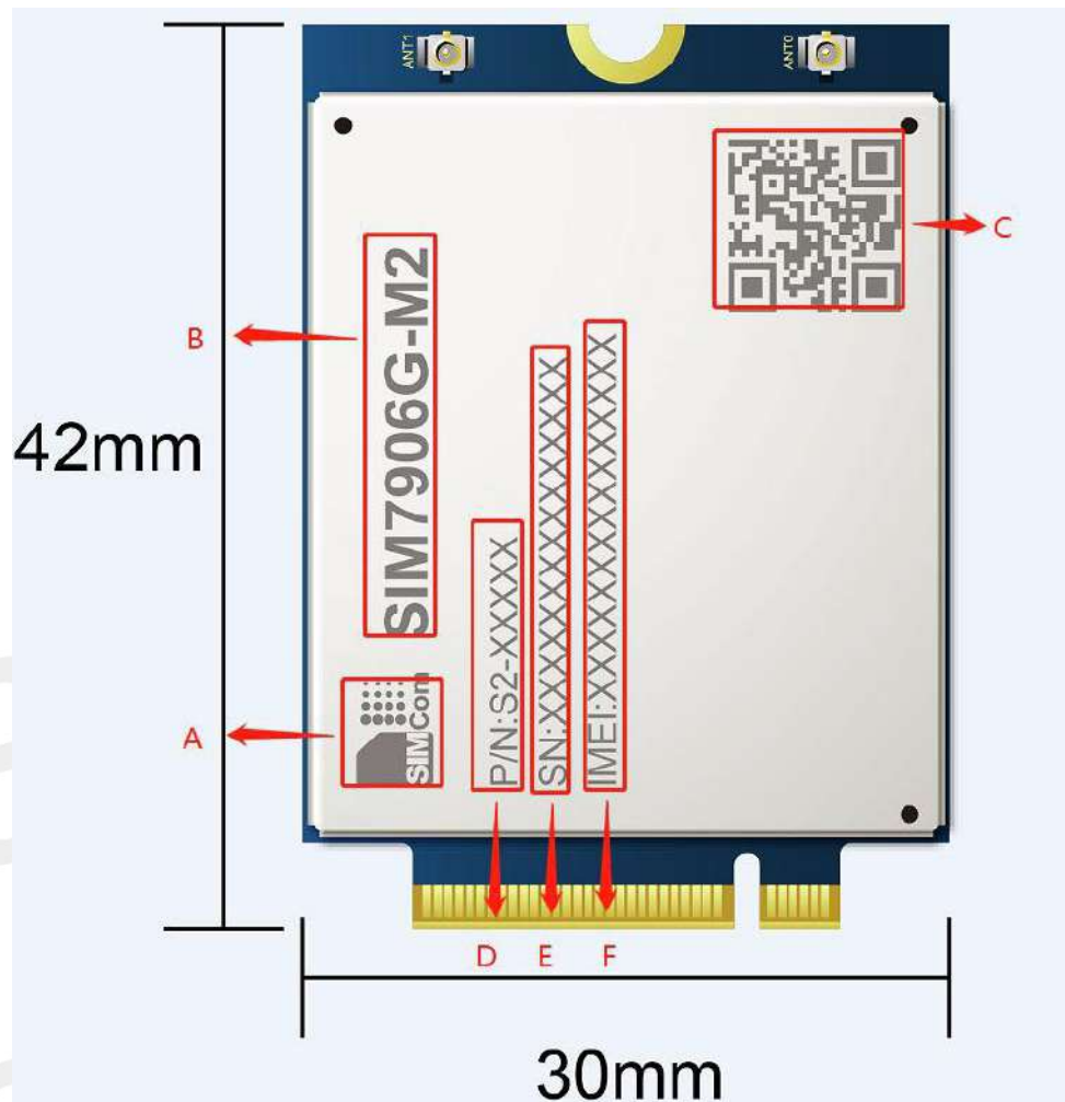
Figure 6: Label information
