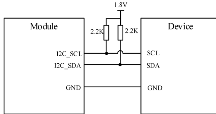
Figure 17: I2C reference circuit
