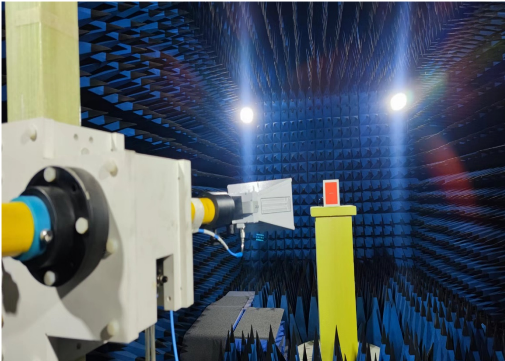
Above 1GHz Test setup
