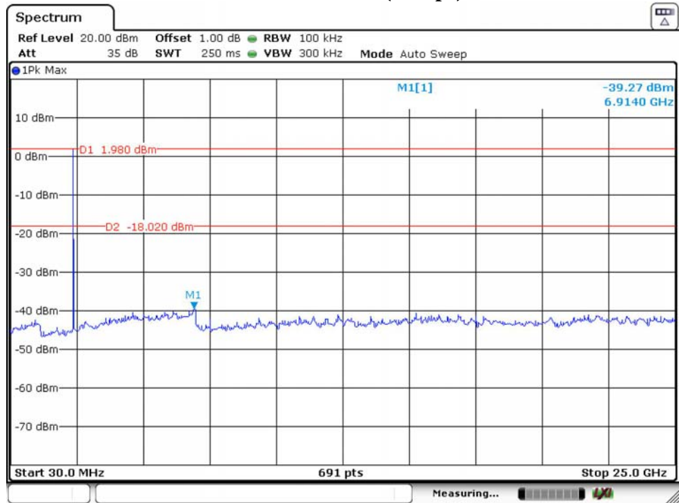
GFSK 2402MHz (2Mbps)
