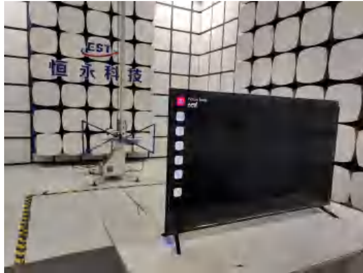
Radiated Test (Below 1GHz)
