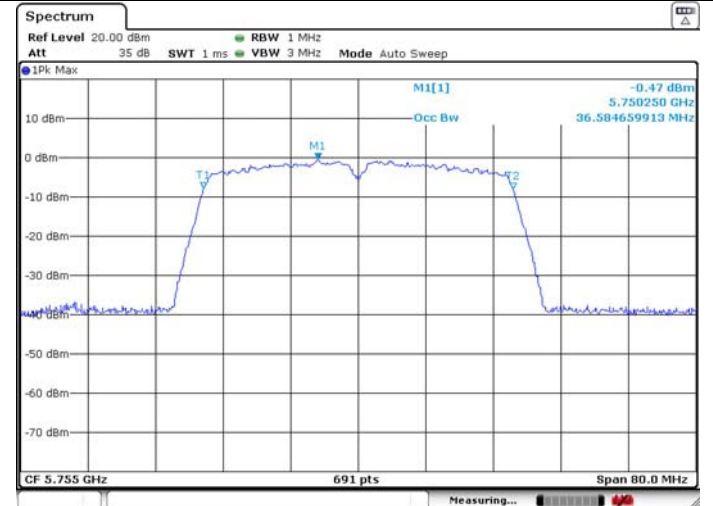
99% Occupied Bandwidth
