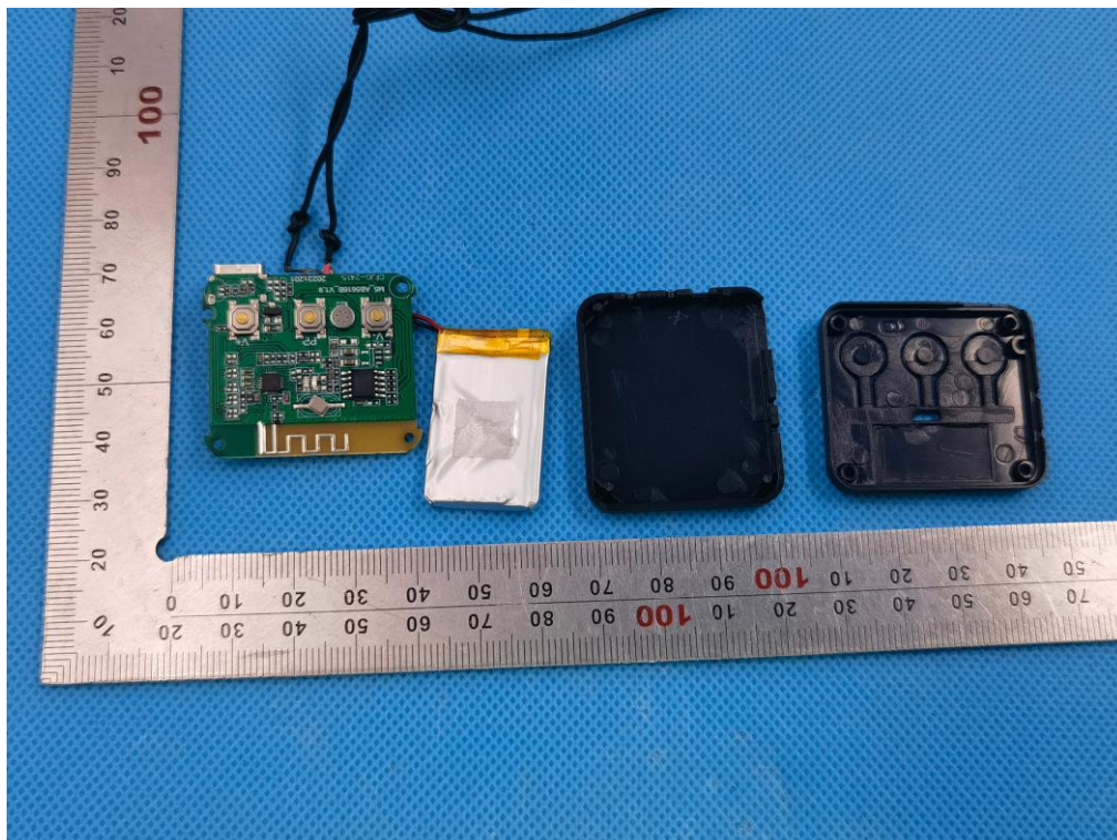
Series Model 5(YX2-B) OPEN VIEW OF EUT (FIGURE 1)
