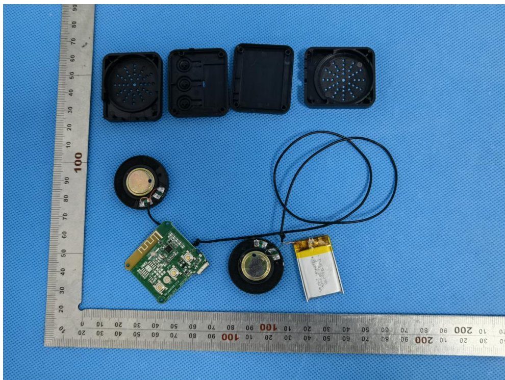
Series Model 2(M1-BL1) OPEN VIEW OF EUT (FIGURE 1)
