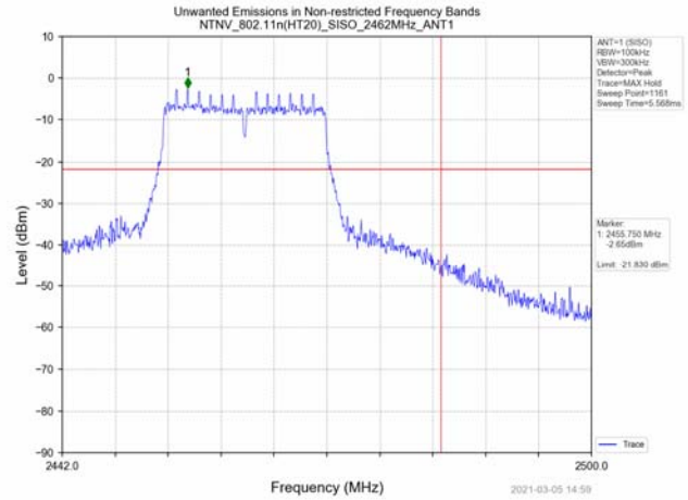
Right bandedge
