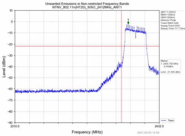
Left bandedge
