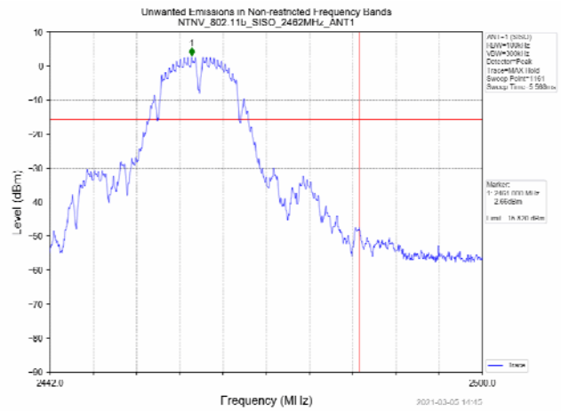
Right bandedge
