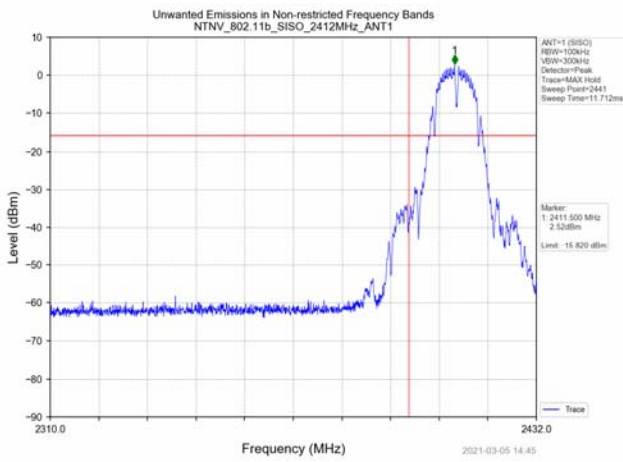
Left bandedge
