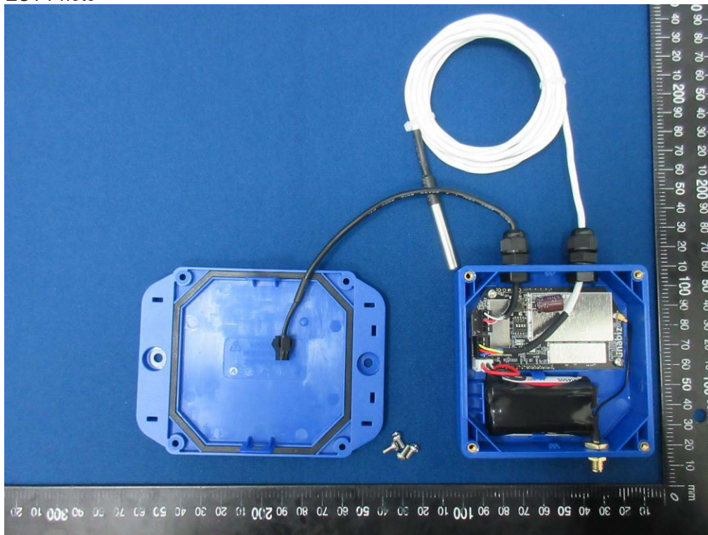
(4) EUT Photo (EVE Battery, Model: F1080B-LF)
