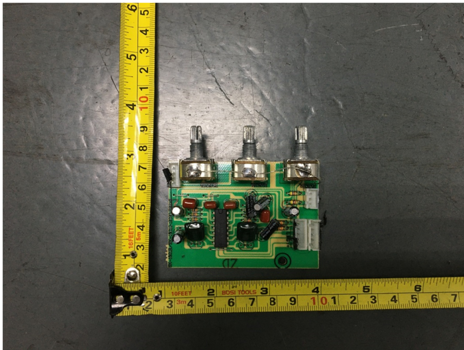
Solder Board-Component View 28
